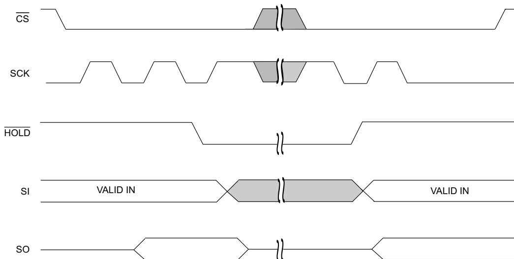
Figure 12. \overline{HOLD} Operation [2]
