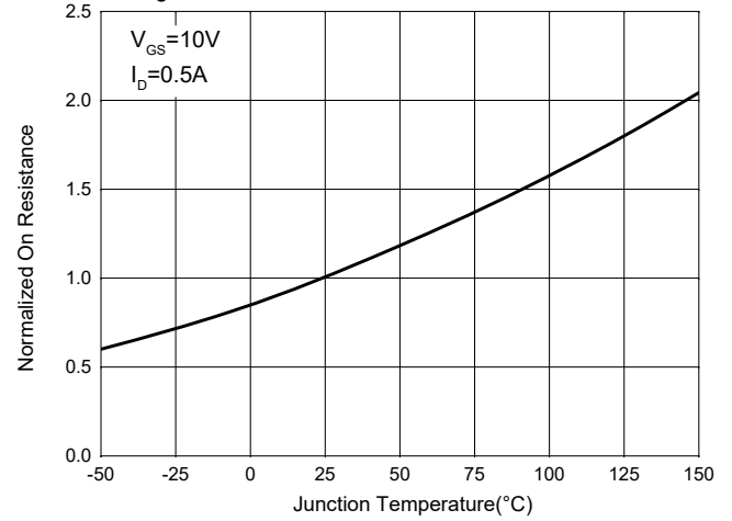
Fig.8-Normalized OnResistanceCharacteristics
