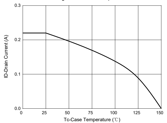
Fig. 10 - Current dissipation
