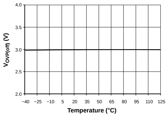
Figure 9. Over-Voltage Protection Threshold ( V_{OVP} Going Up), V_{OVP(off)}
