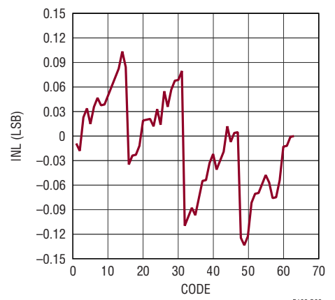
Integral Nonlinearity
