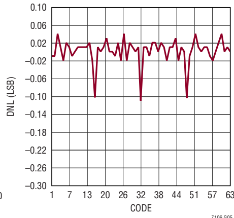
Differential Nonlinearity
