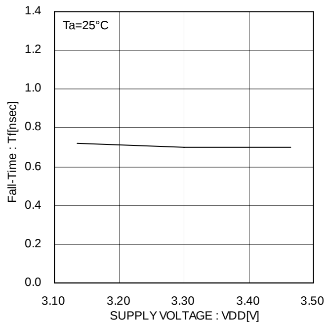
Figure 23. CLKOUT Fall-Time
