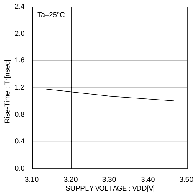
Figure 21. CLKOUT Rise-Time
