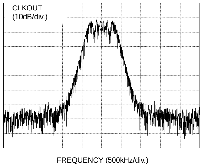
Figure 26. CLKOUT±0.50% Modulation Spectrum
