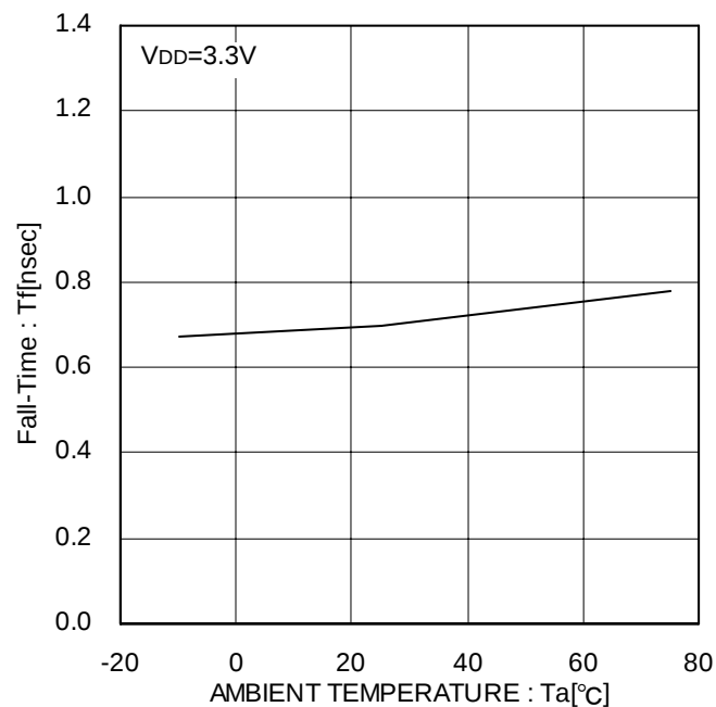
Figure 24. CLKOUT Fall-Time
