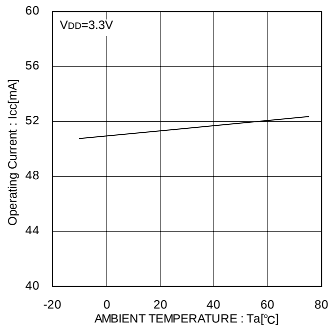
Figure 46. Operating Current
