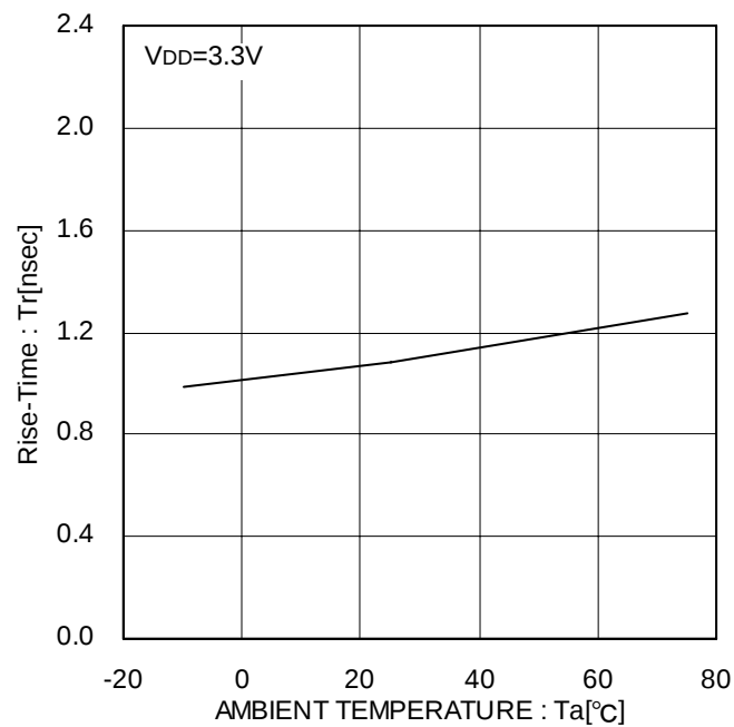
Figure 22. CLKOUT Rise-Time
