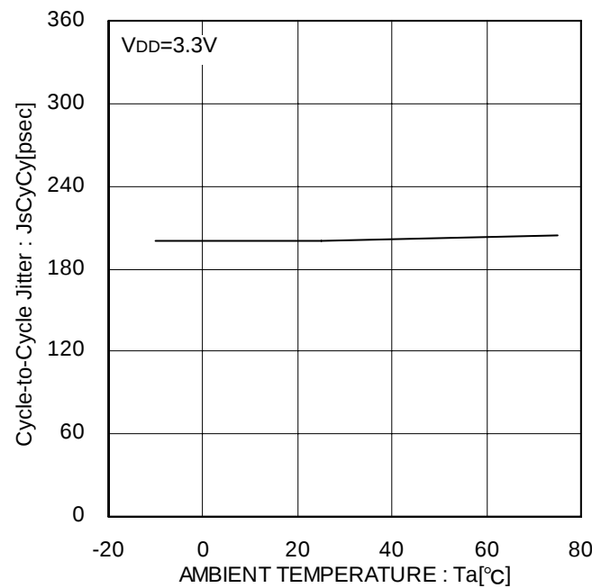
Figure 38. CLKOUT ±0.25% Modulation Cycle-to-Cycle Jitter
