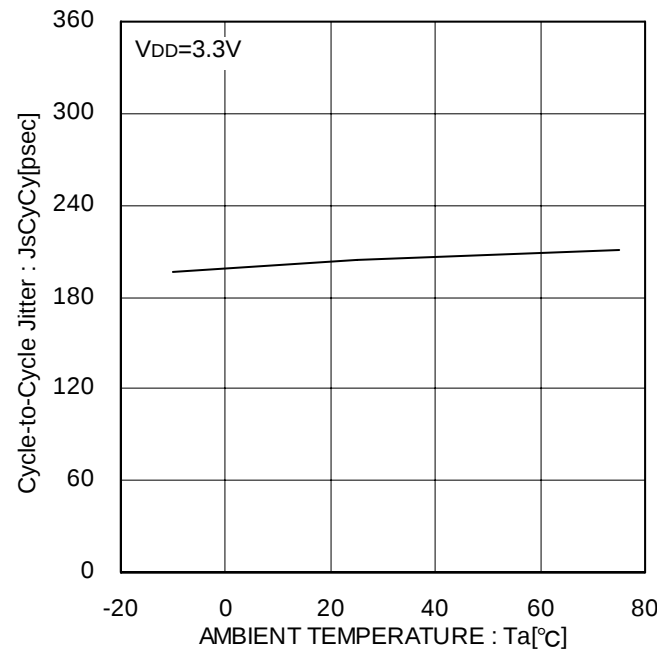
Figure 40. CLKOUT ±0.50% Modulation Cycle-to-Cycle Jitter
