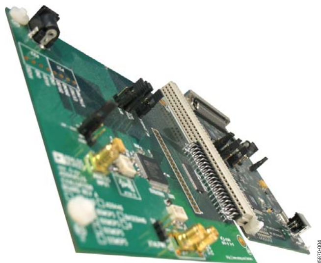
Figure 4. Single-Channel ADC
