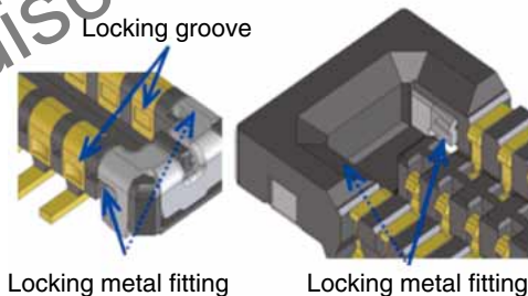
Fig.1. Geometry of the contact locking groove and the locking metal fitting
