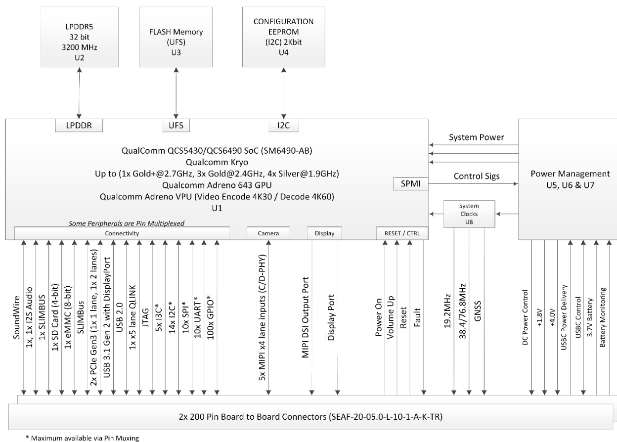
Figure 1 MitySOM-QC Block Diagram
