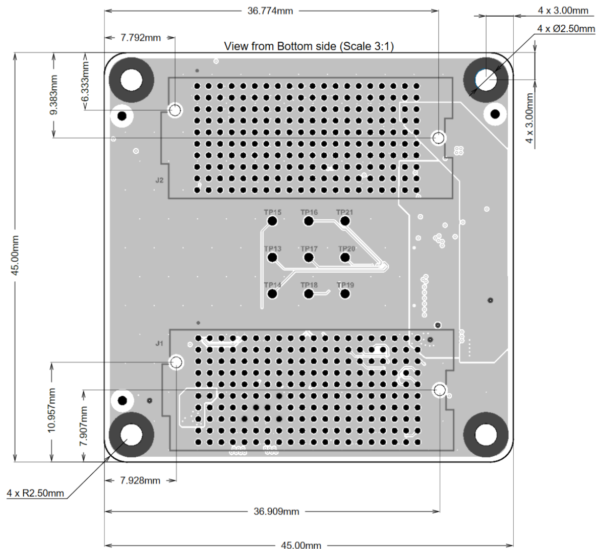
Figure 4: MitySOM-QC Mechanical Outline, View From Bottom
