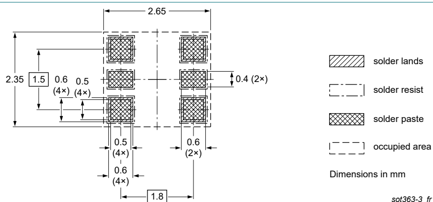
Fig. 14. Reflow soldering footprint for TSSOP6 (SOT363-3)
