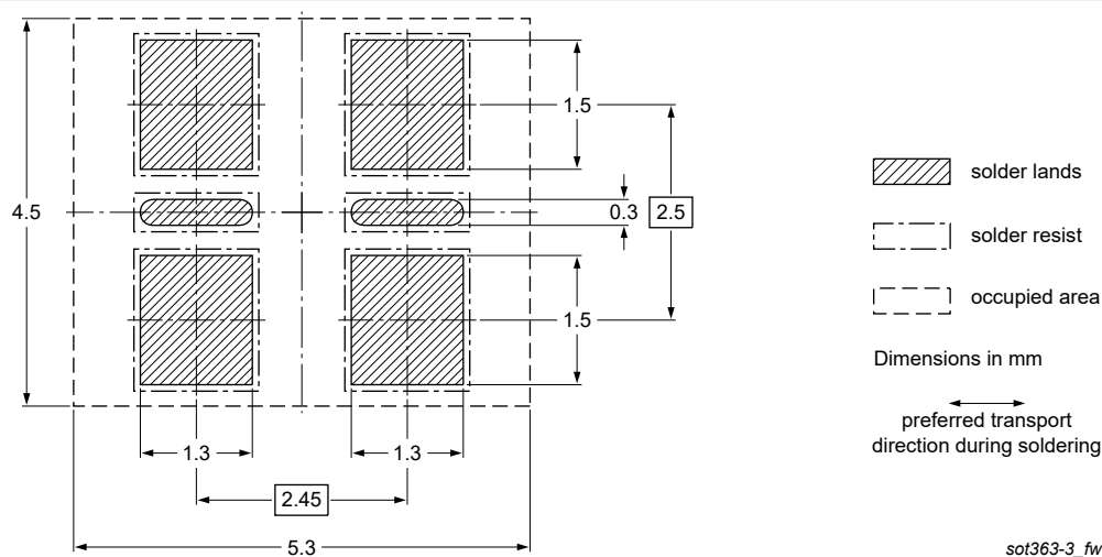
Fig. 15. Wave soldering footprint for TSSOP6 (SOT363-3)
