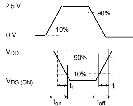
(c) V_{OUT}
