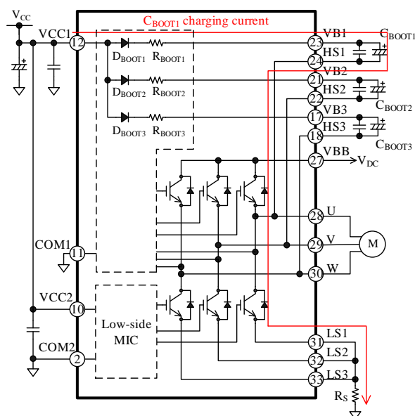
Figure 12-1. Bootstrap Circuit
