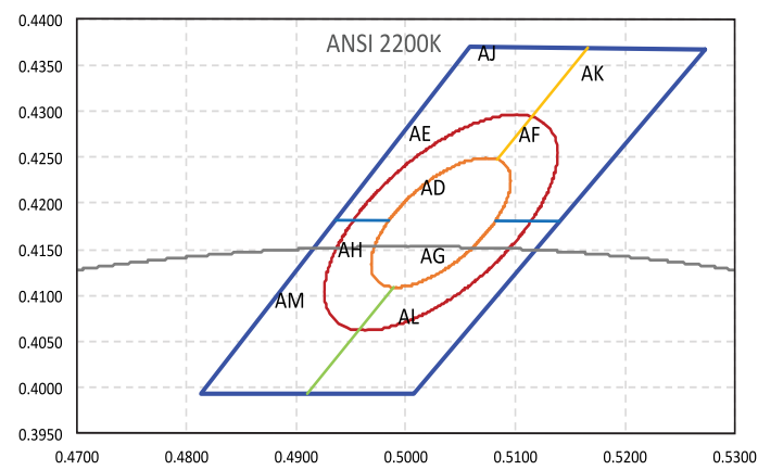
Figure 8a. Color bin structure for LUXEON 3014 2200K, hot-color targeted at T j =65°C.
