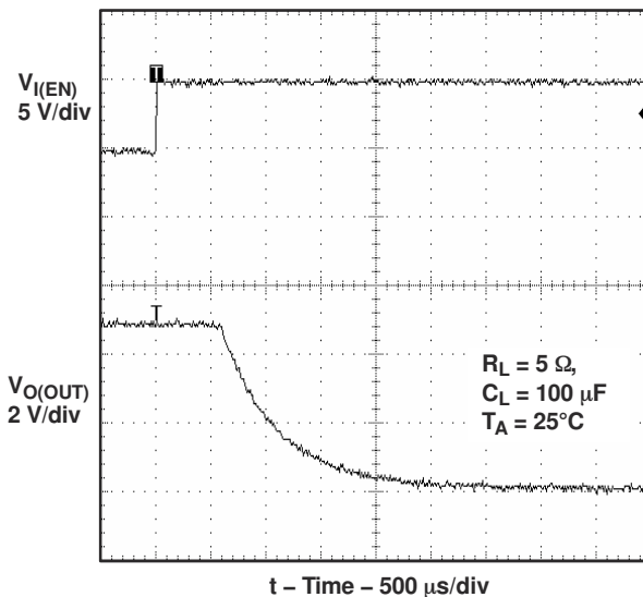
Figure 7-19. Turnoff Delay and Fall Time With 100-μF Load
