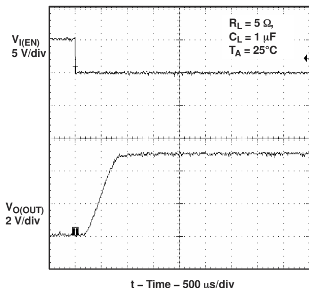
Figure 7-16. Turnon Delay and Rise Time With 1- \mu F Load
