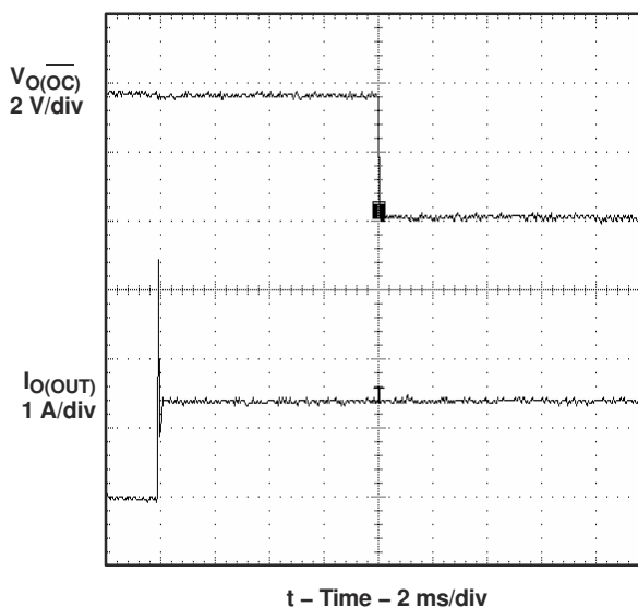
Figure 7-23. 1-Ω Load Connected to Enabled Device
