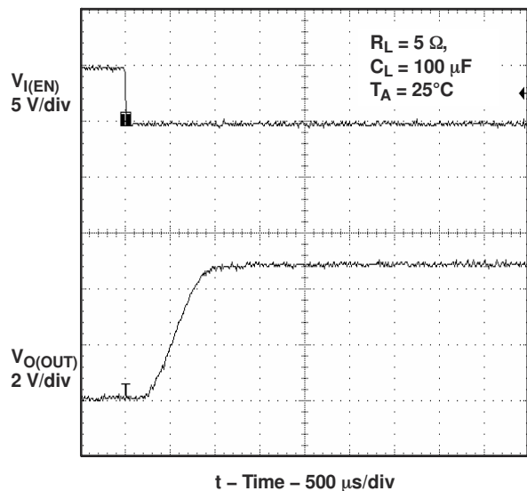
Figure 7-18. Turnon Delay and Rise Time With 100-μF Load
