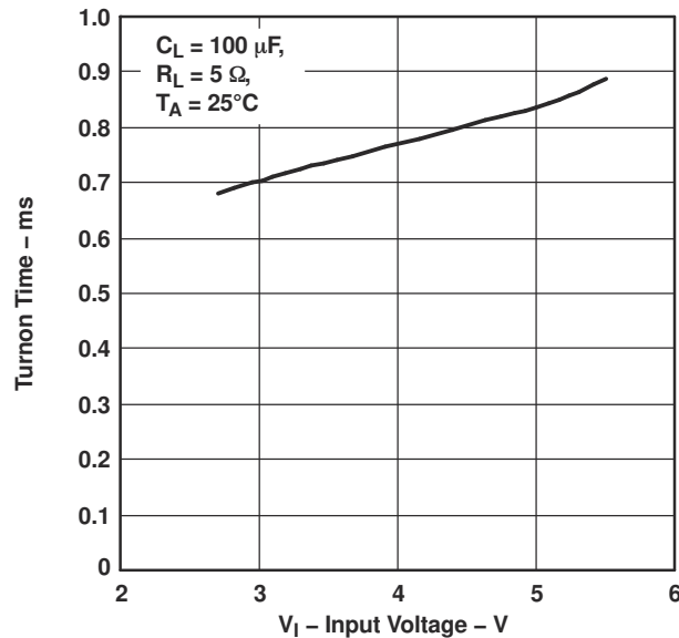
Figure 7-1. TURNON TIME vs INPUT VOLTAGE
