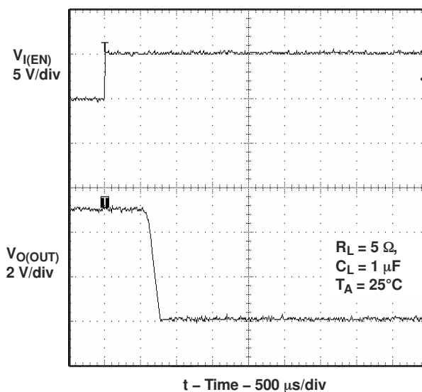
Figure 7-17. Turnoff Delay and Fall Time With 1- \mu F Load
