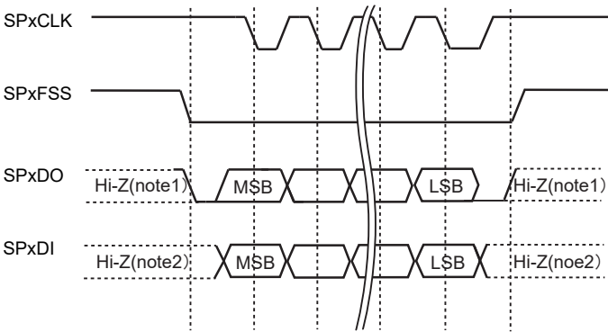
Figure 21-7 SPI frame format (single transfer, <SPO>="1" & <SPH>="0")
