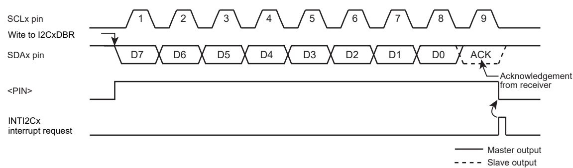
Figure 20-11 <BC[2:0]>= "000",<ACK>= "1" (Transmitter Mode)
