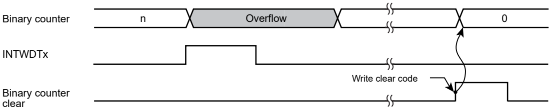
Figure 25-2 INTWDTx interrupt generaiton
