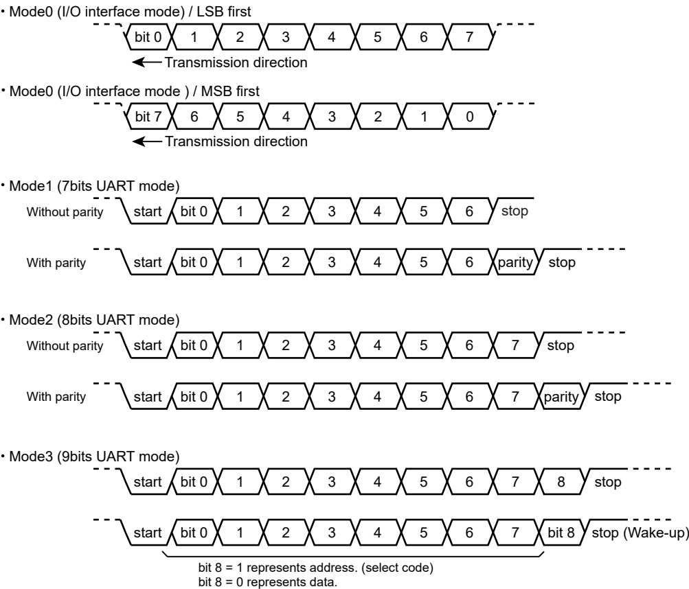
Figure 18-3 Data Format
