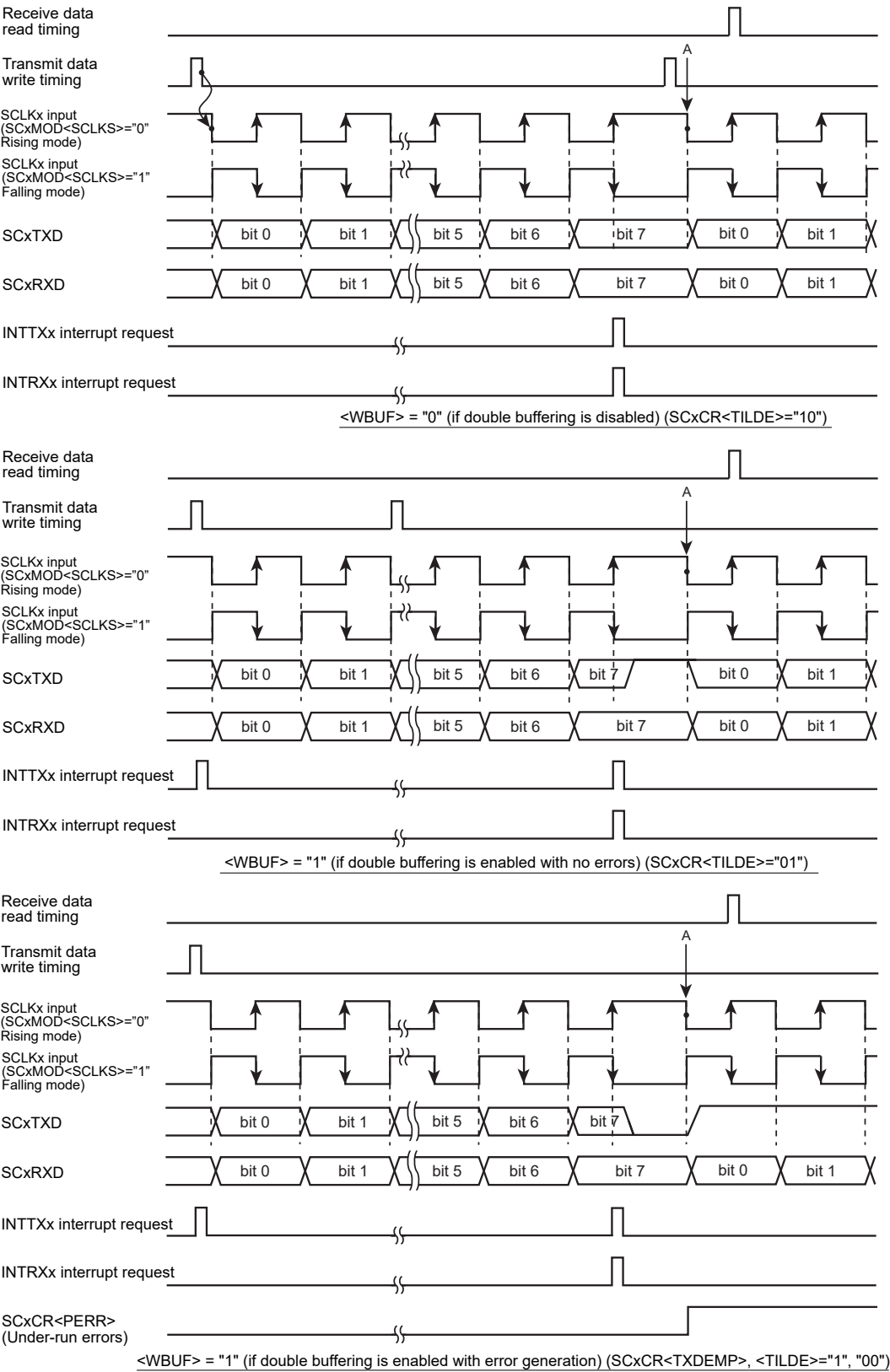
Figure 18-20 Transmit/Receive Operation in the I/O Interface Mode (Clock Input Mode)
