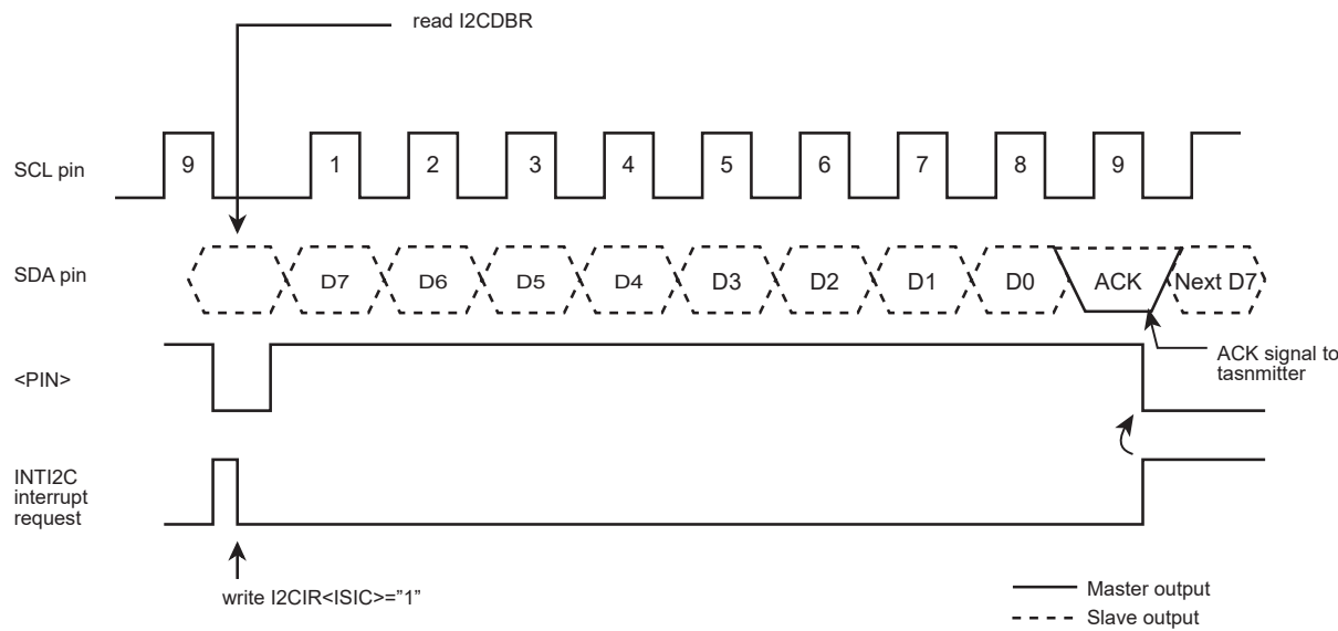
Figure 20-12 <BC[2:0]>= "000",<ACK>= "1" (Receiver Mode)
