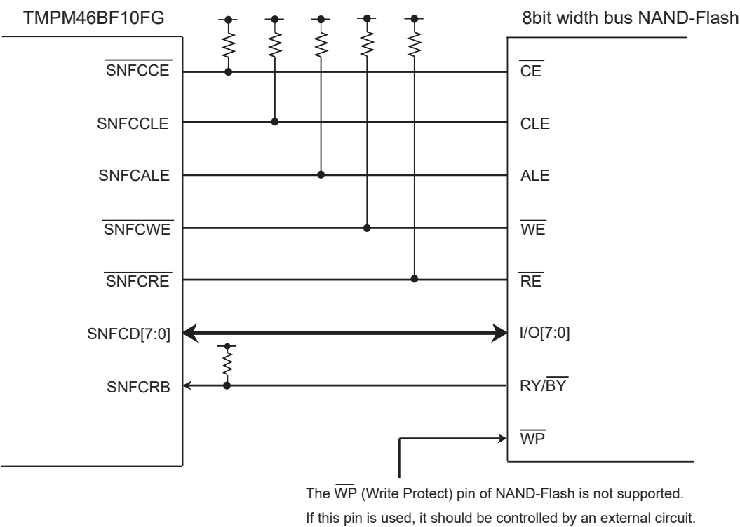
Figure 11-5 Connection Example
