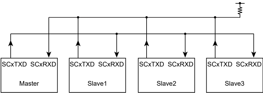
Figure 18-21 Serial Links to Use Wake-up Function
