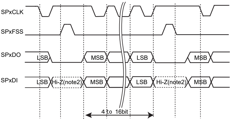
Figure 21-8 SPI frame format (continuous transfer, <SPO>="1" & <SPH>="0")
