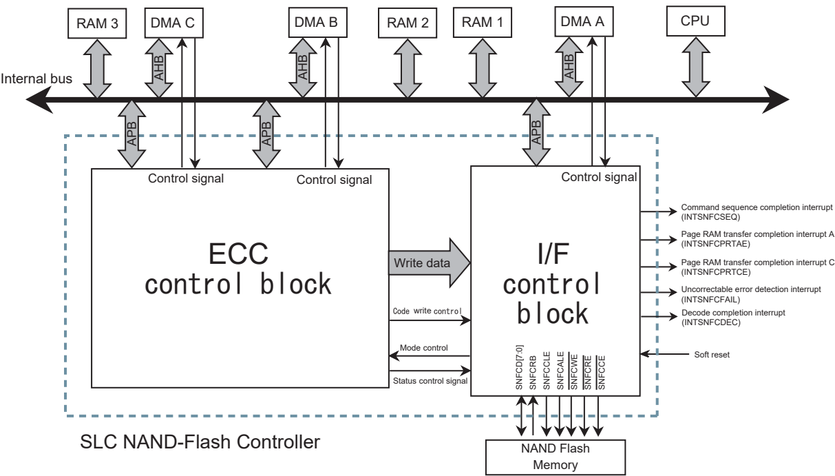
Figure 11-2 SLC NAND flash controller and Peripheral Functions
