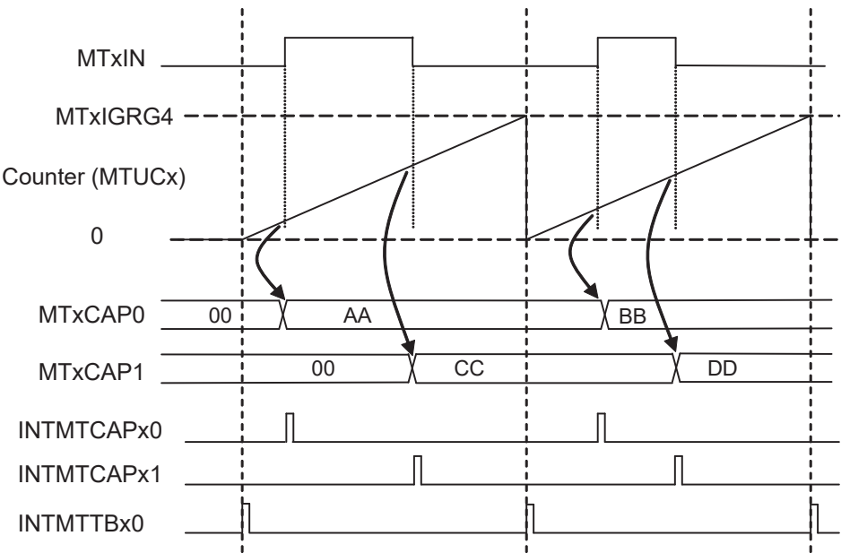
Figure 17-10 Capture operation
