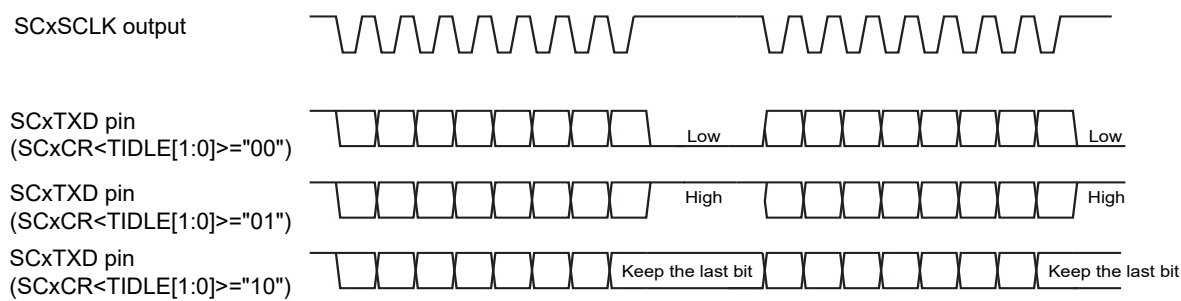
Figure 18-9 Level of SCxTXD pin After the last bit is output
