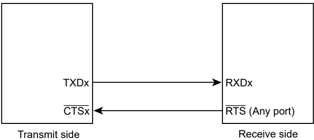
Figure 18-11 Handshake Function
