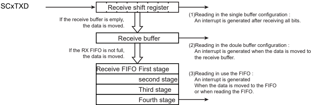
Figure 18-13 Receive Buffer/FIFO Configuration Diagram
