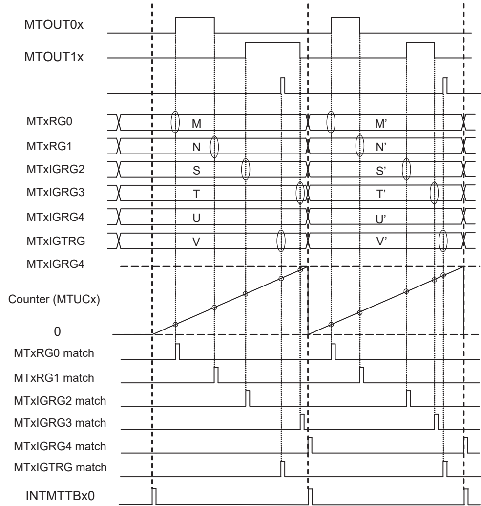
Figure 17-8 IGBT mode basic timing
