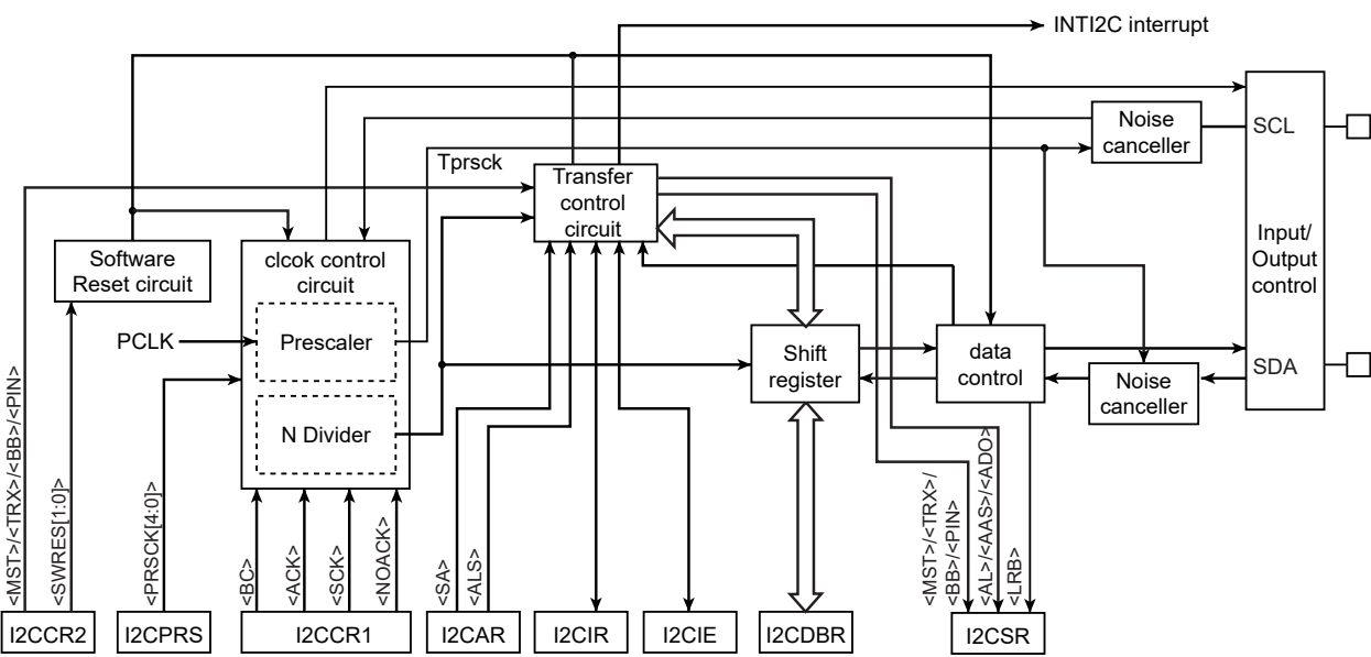
Figure 20-1 I2C Bus Block
