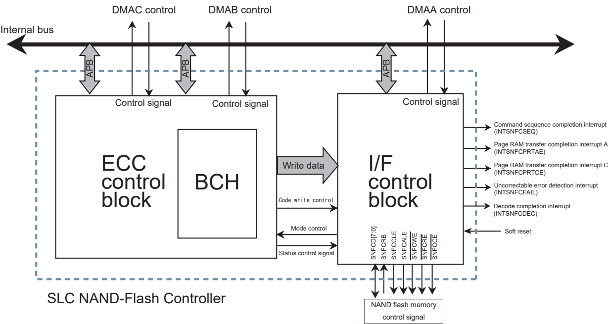
Figure 11-1 Block diagram
