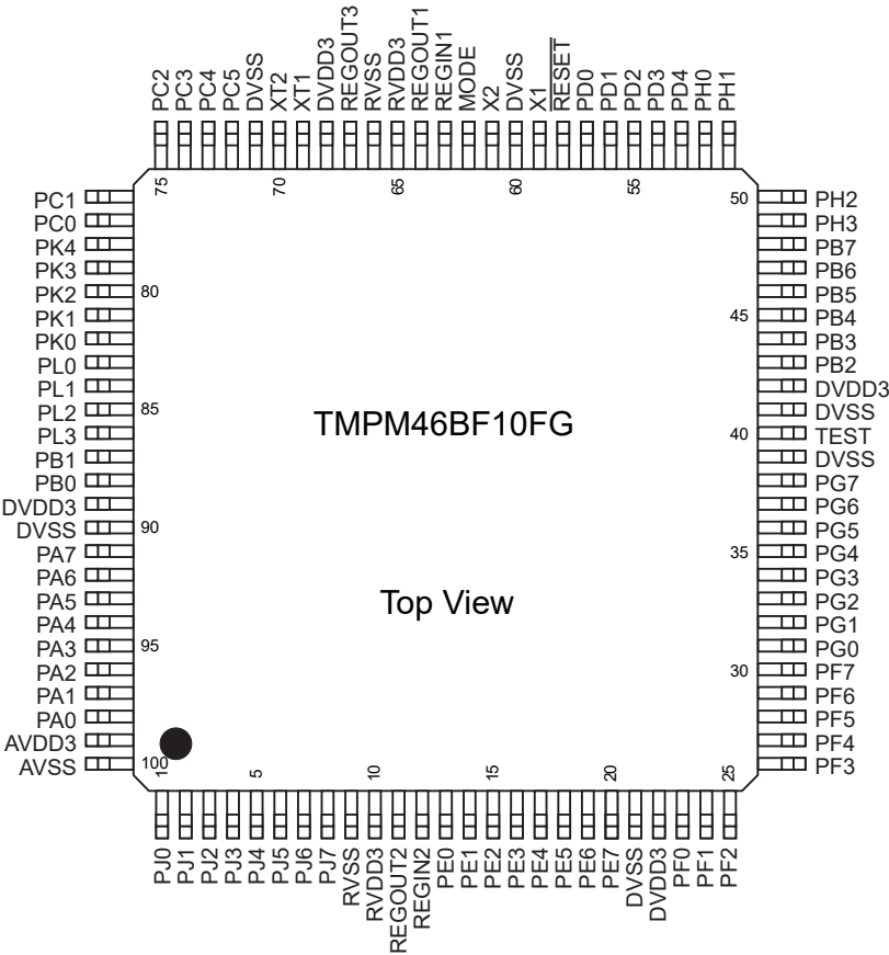
Figure 1-2 Pin Layout (LQFP100 TOP VIEW)
