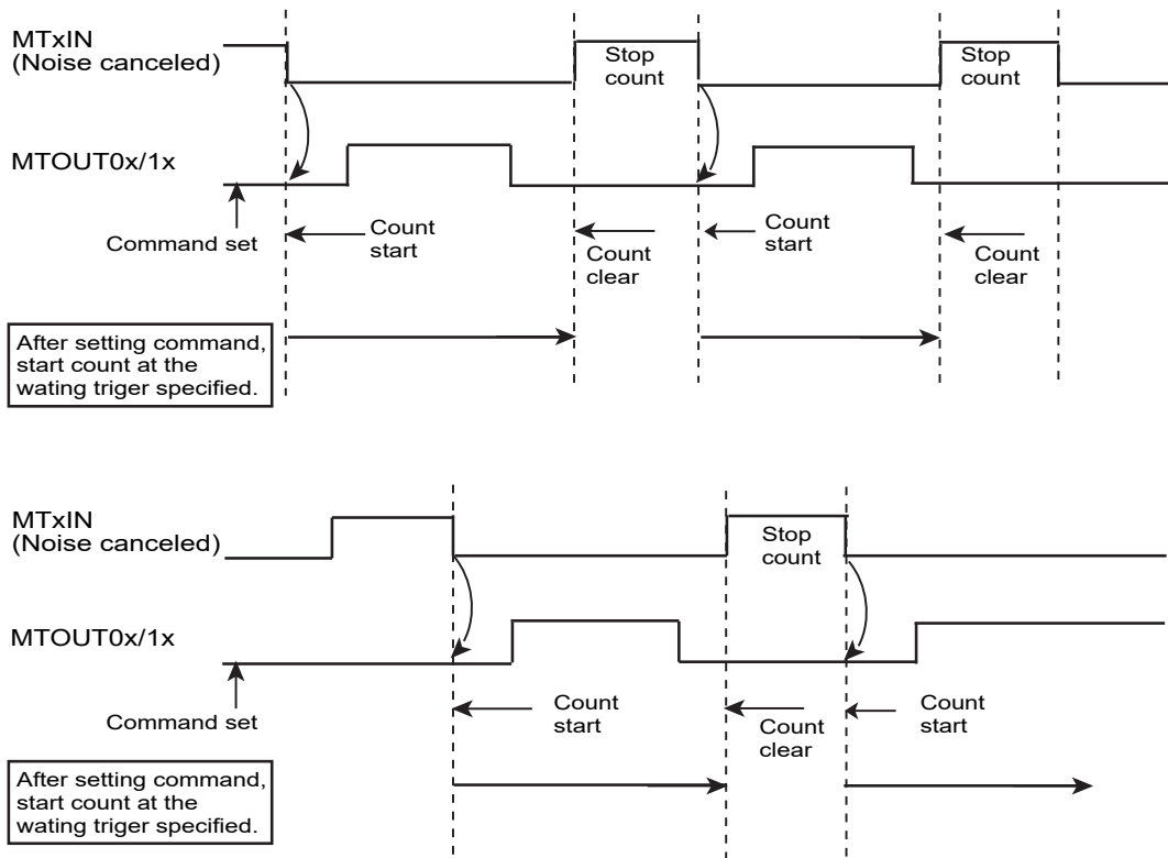
Figure 17-12 Trigger Start
