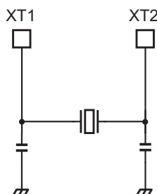
Figure 29-2 Low-frequency oscillation connection
