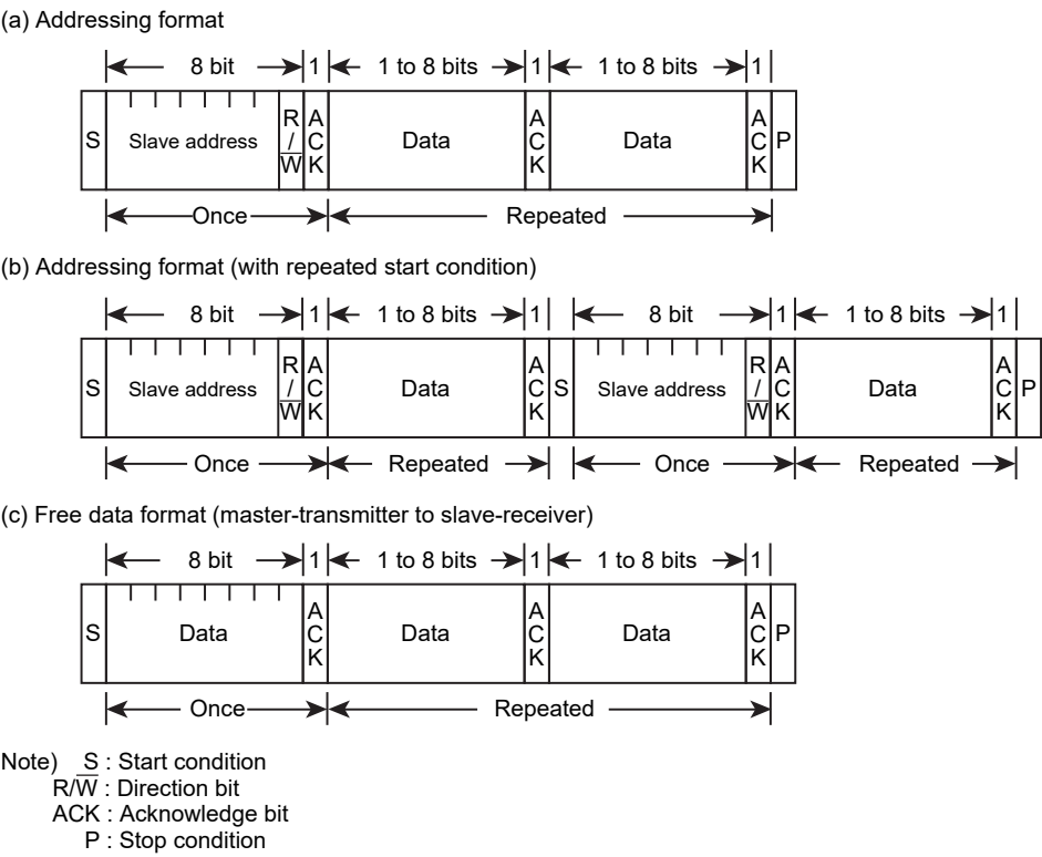
Figure 20-3 I2C Bus Mode Data Formats
