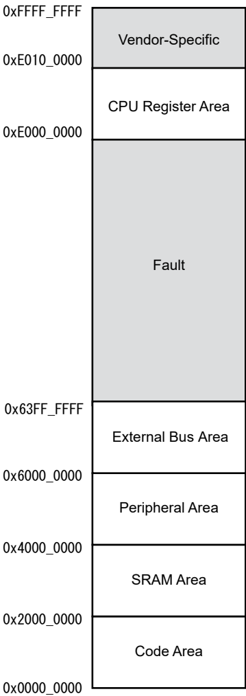
Figure 4-1 MemoryMap
