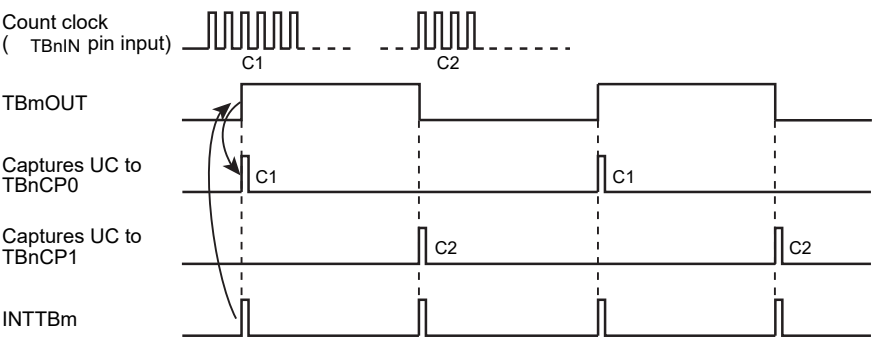
Figure 16-6 Frequency measurement
