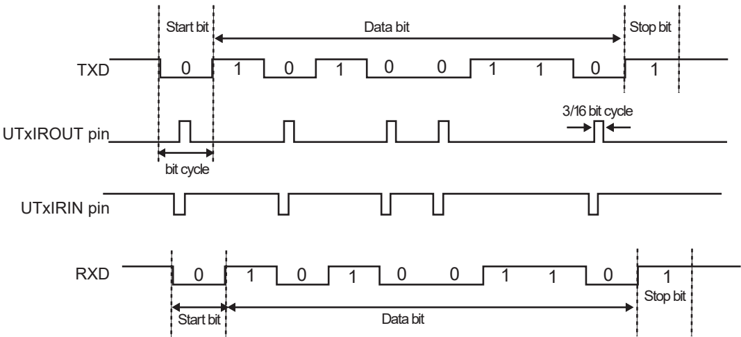
Figure 19-4 IrDA Data Modulation
