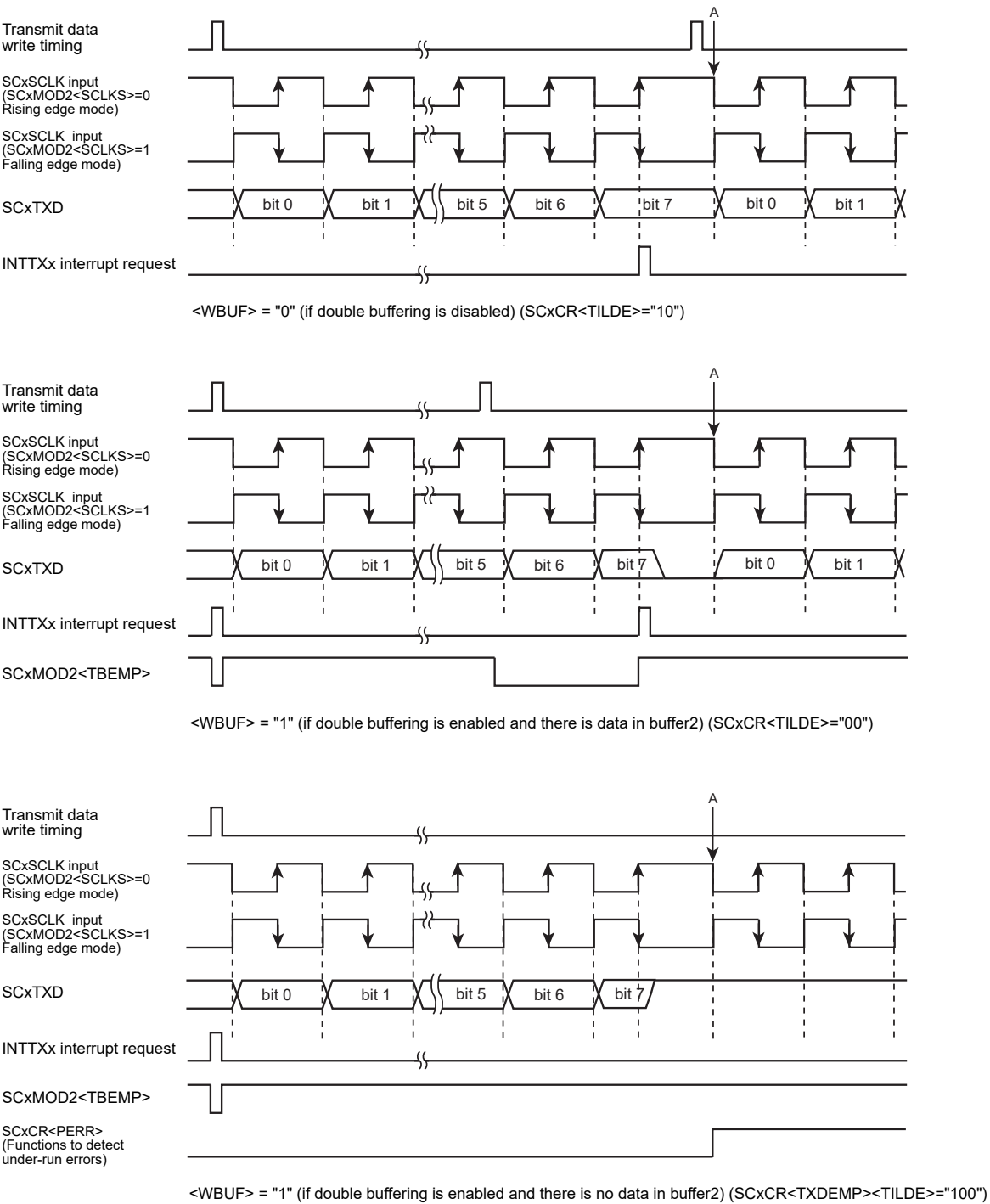
Figure 18-16 Transmit Operation in the I/O Interface Mode (Clock Input Mode)
