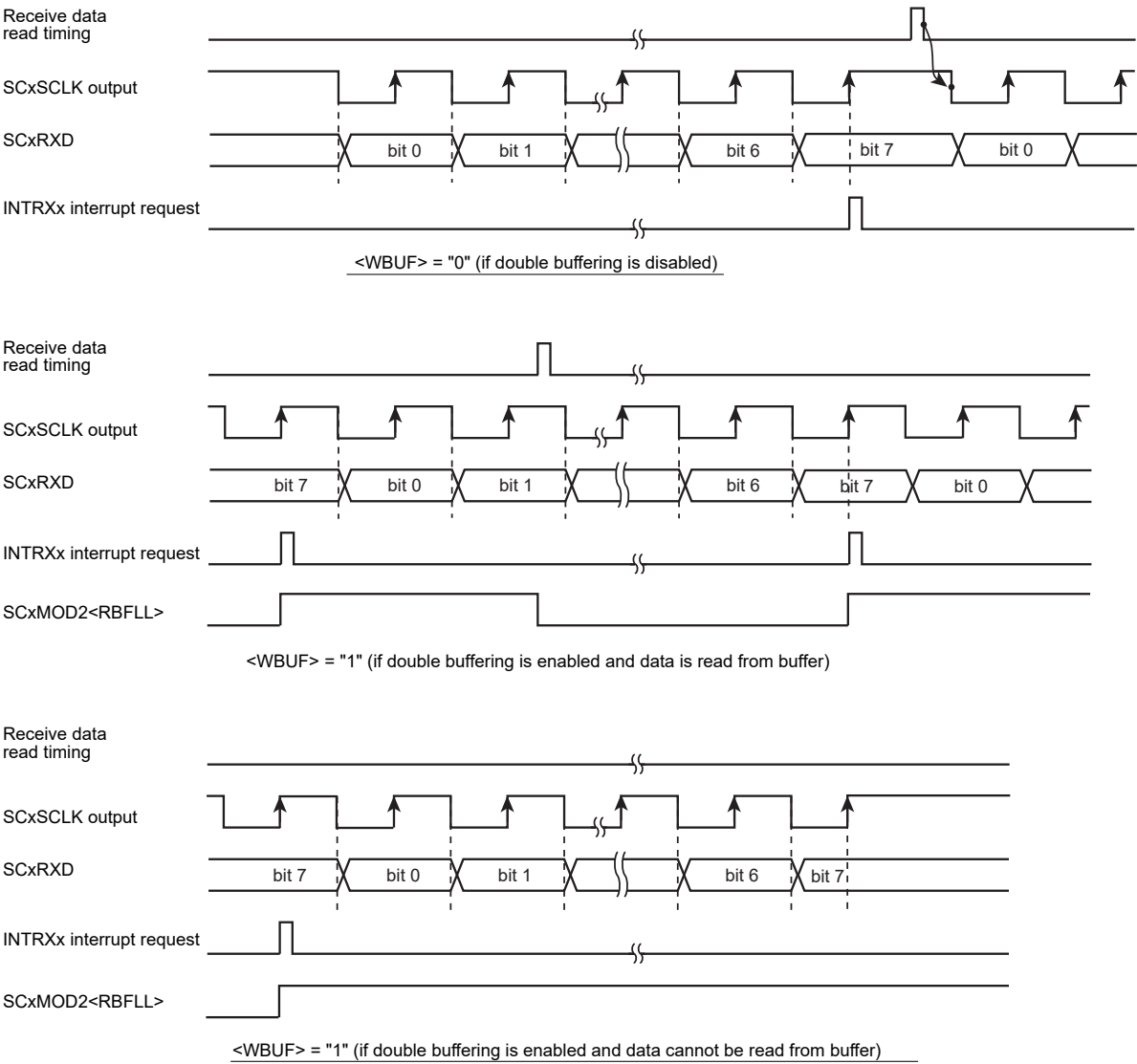
Figure 18-17 Receive Operation in the I/O Interface Mode (Clock Output Mode)
