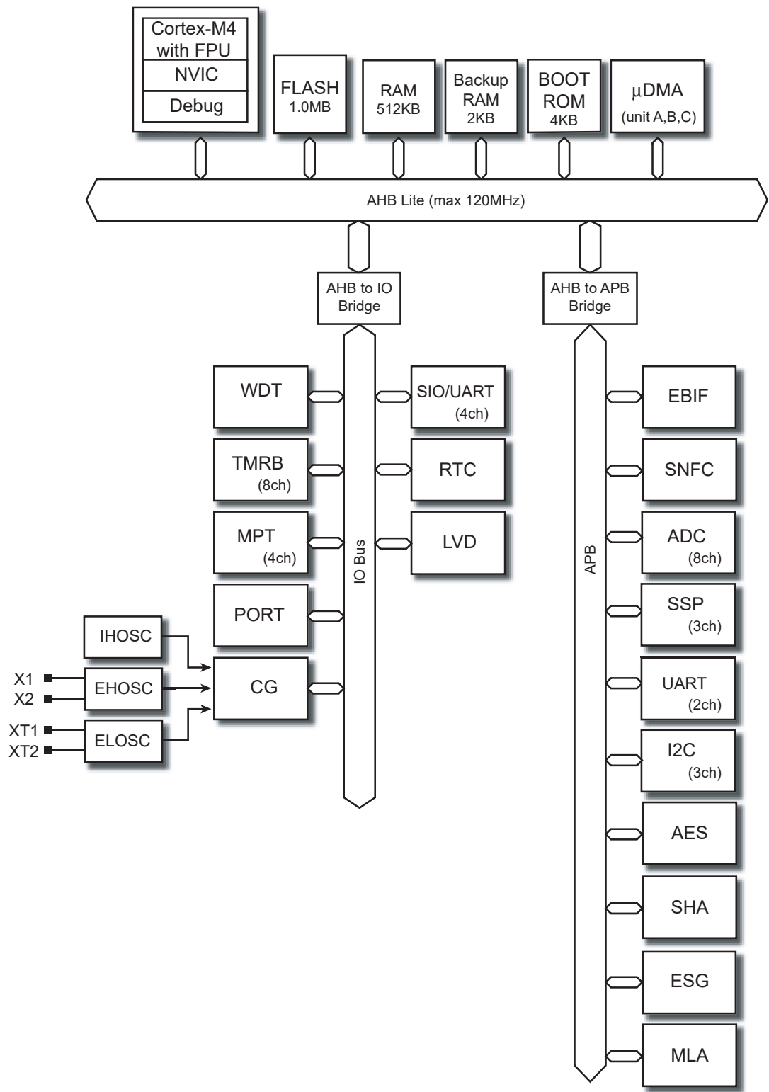
Figure 1-1 Block Diagram
