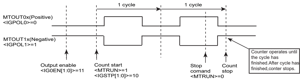
Figure 17-17 Counter stops with initial state after cycle has finished
