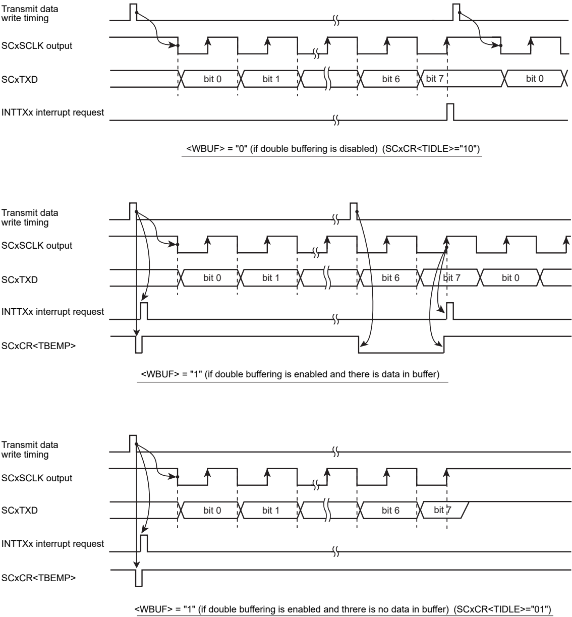
Figure 18-15 Transmit Operation in the I/O Interface Mode (Clock Output Mode)
