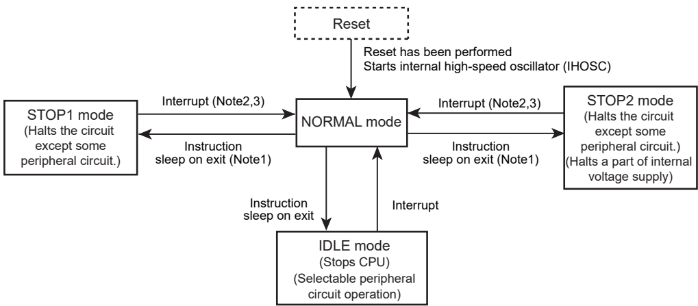
Figure 6-2 Mode Transition Diagram
