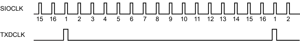
Figure 18-7 Generation of Transmission Clock in UART mode
