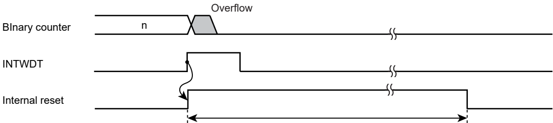
Figure 25-3 Internal reset generation
