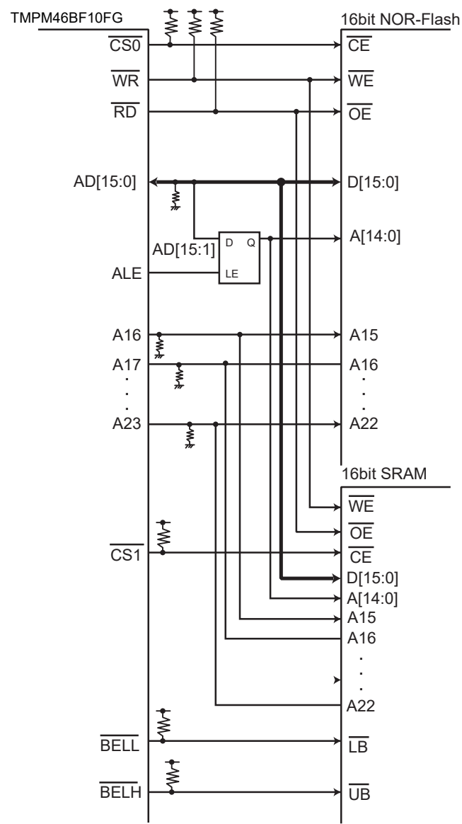
Figure 10-10 Connection Example of external 16-bit SRAM and NOR-Flash (Non-synchronous Multiplex mode)
