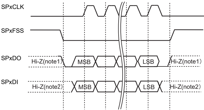
Figure 21-4 SPI frame format (single transfer, <SPO>="0" & <SPH>="0")
