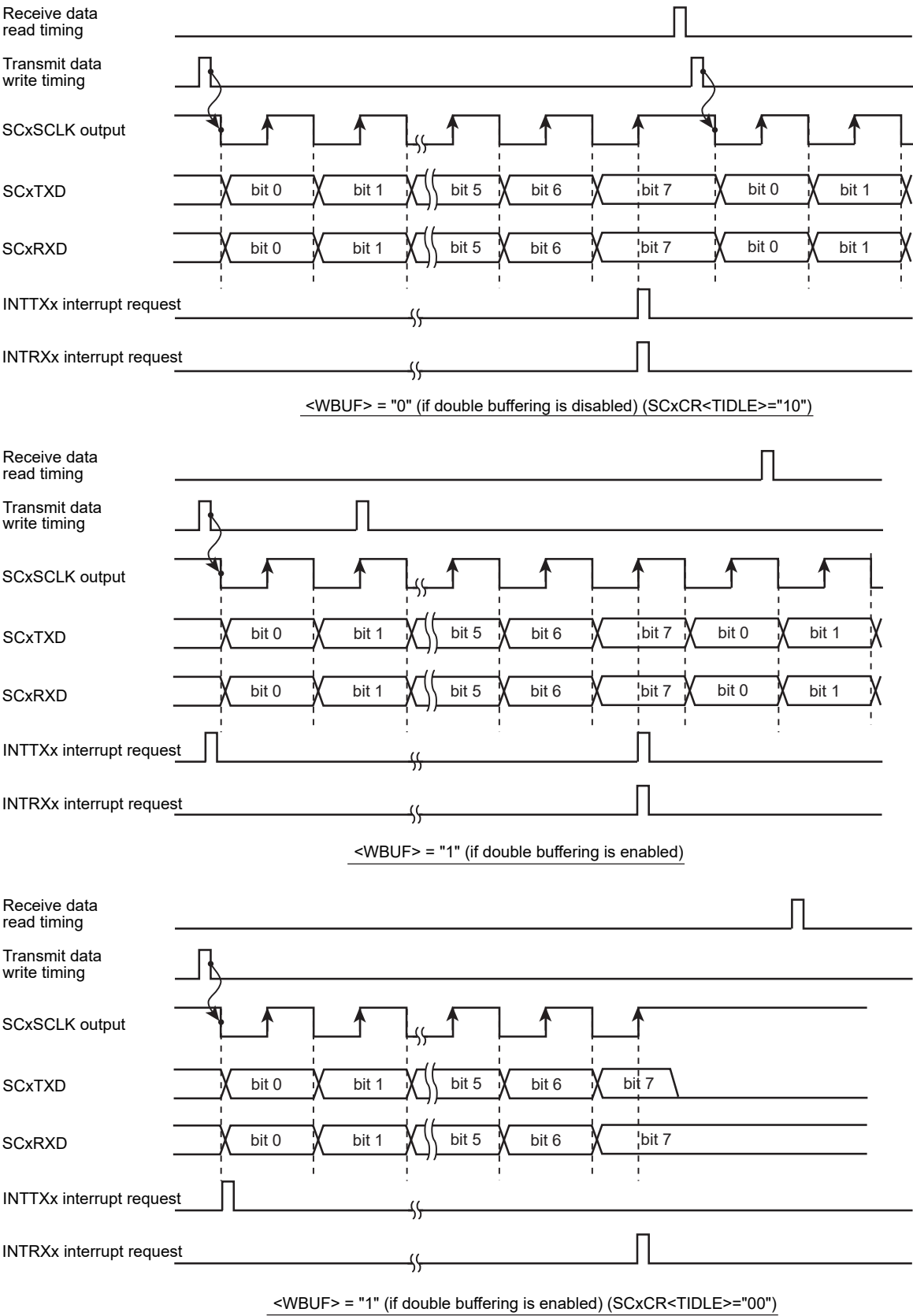
Figure 18-19 Transmit/Receive Operation in the I/O Interface Mode (SCLK Output Mode)
