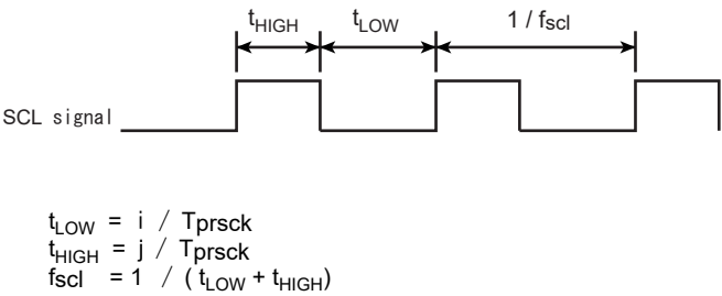
Figure 20-4 Clock source
