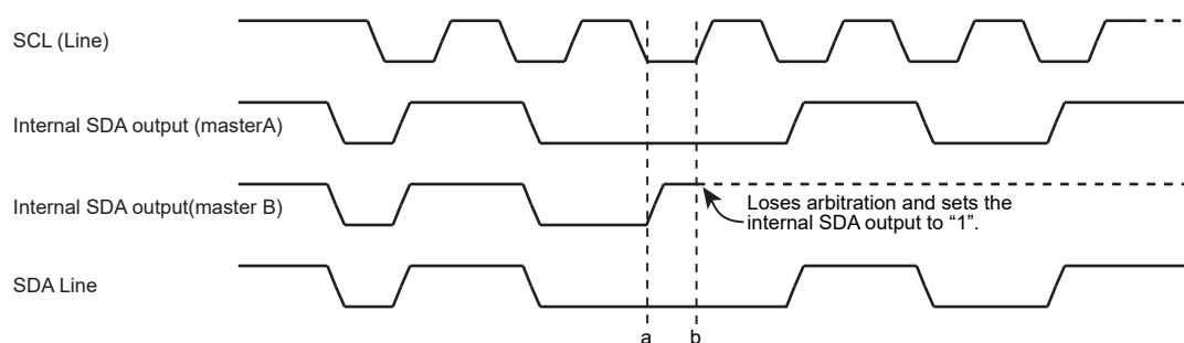
Figure 20-8 Lost Arbitration
