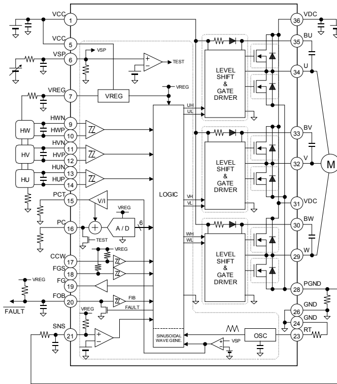
Figure 2. Block Diagram
