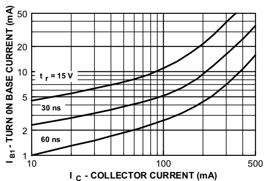
Figure 9. Rise Time vs. Turn-On Base Current
