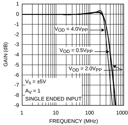
Figure 3. Frequency Response vs V_{OD}
