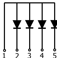
"DAP" common anodes / gemeinsame Anoden
