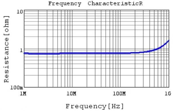
DE11XRA100KA4BQ01F R DC0V, 20degC
