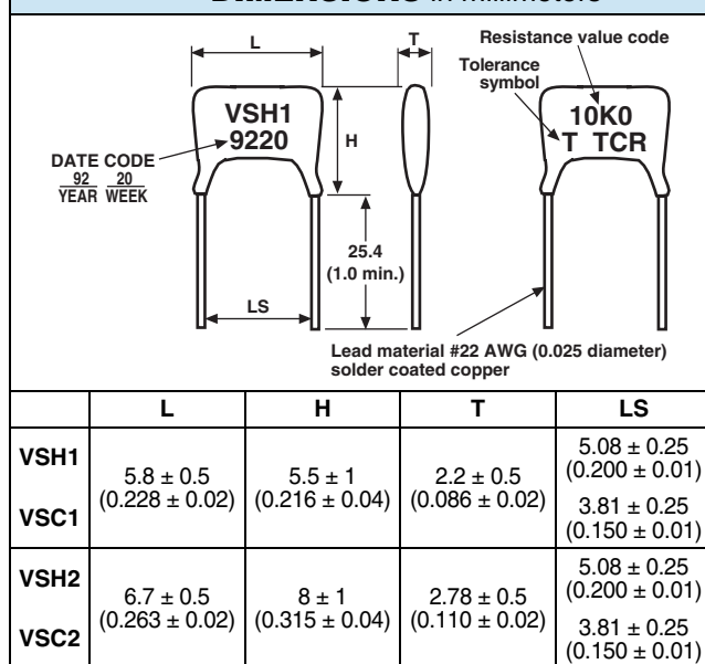
FIGURE 1 - STANDARD IMPRINTING AND DIMENSIONS in millimeters
