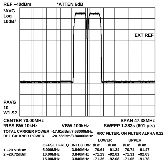
Figure 16. Two-Carrier WCDMA at 400 MSPS f_{OUT} = 70 MHz
