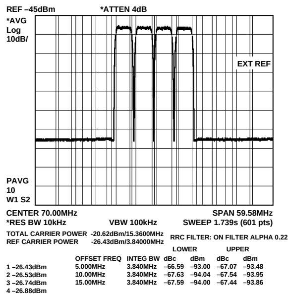
Figure 17. Four-Carrier WCDMA at 400 MSPS f_{OUT} = 70 MHz
