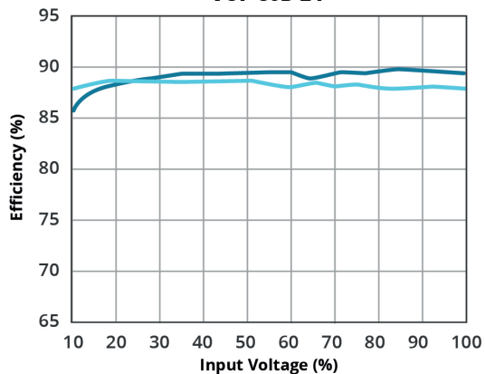
EFFICIENCY VS INPUT LOAD VOF-80B-24
