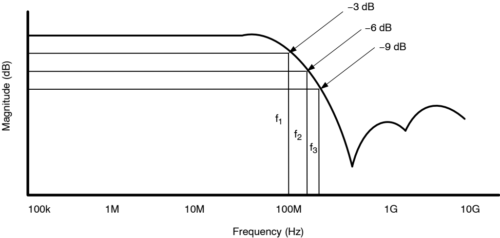
Figure 5. Filter Bandwidth
