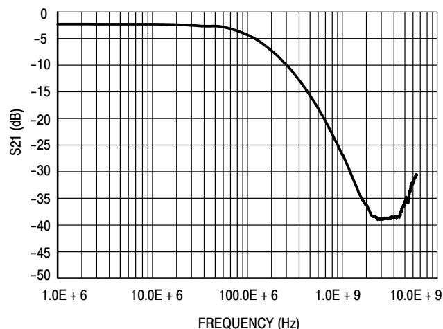
Figure 2. Typical Insertion Loss Characteristics (S21 Measurement)
