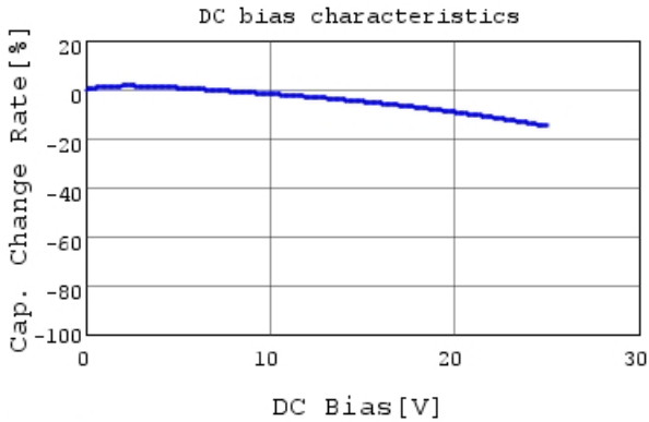
GRM155R71E222KA01 C-DC bias capchange, 25.0c
