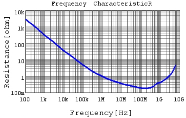
GRM155R71E222KA01 R DCOV, 25degC
