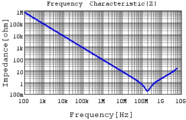
GRM155R71E222KA01 |Z| DCOV, 25degC
