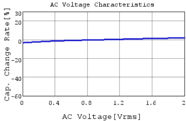
GRM155R71E222KA01 C-AC Voltage capchange, Dc
