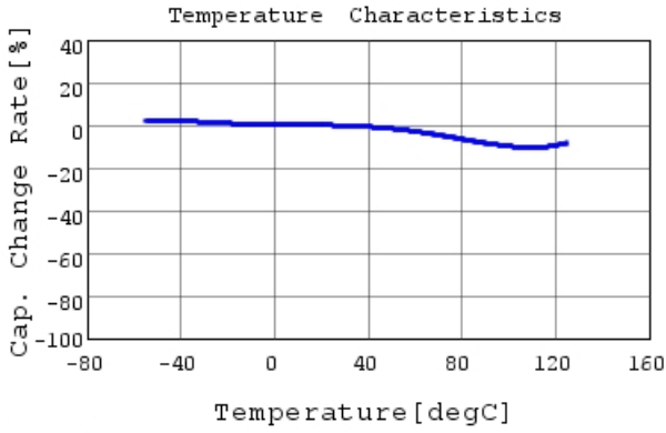
GRM155R71E222KA01 C-Temp. capchange, DC0.0V,
