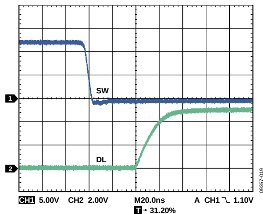
Figure 19. Low-Side Driver Rising Edge Waveform, C DL = 2.2 nF
