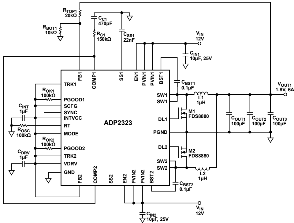
Figure 52. Parallel Single Output Application, V_{IN} = 12V , V_{OUT} = 1.8V , I_{OUT} = 6A , f_{SW} = 600kHz
