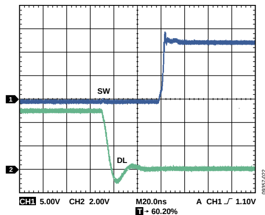
Figure 22. Low-Side Driver Falling Edge Waveform, C DL = 2.2 nF
