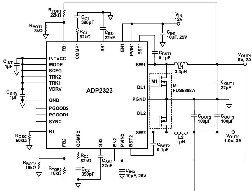
Figure 53. Cascading Supply Application, V_{IN1} = 12V , V_{OUT1} = 5V , I_{OUT1} = 2A , V_{OUT2} = 1V , I_{OUT2} = 3A , f_{SW} = 1.2MHz
