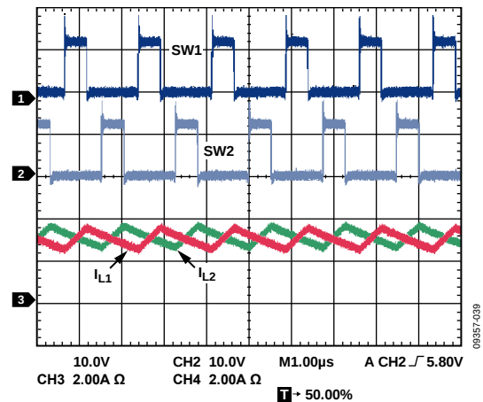
Figure 39. Dual Phase, Single Output, V_{OUT} = 3.3\text{ V} , I_{OUT} = 6\text{ A}
