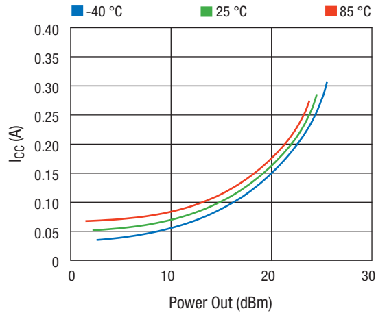
Figure 27. Icc vs Power Out Across Temperature
