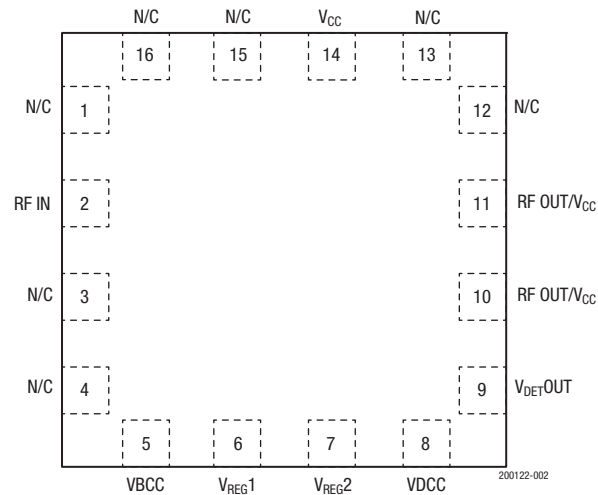
Figure 2. SKY65006-348LF Pinout
