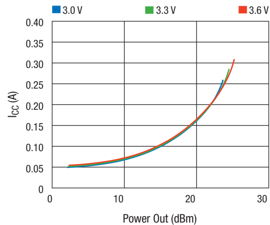
Figure 29. Icc vs Power Out Across Vcc
