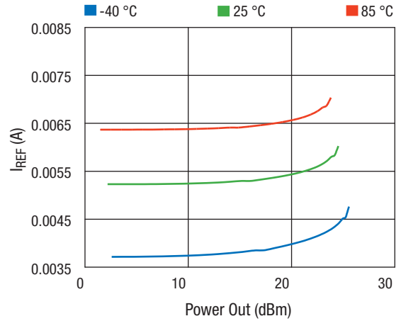
Figure 28. Iref vs Power Out Across Temperature
