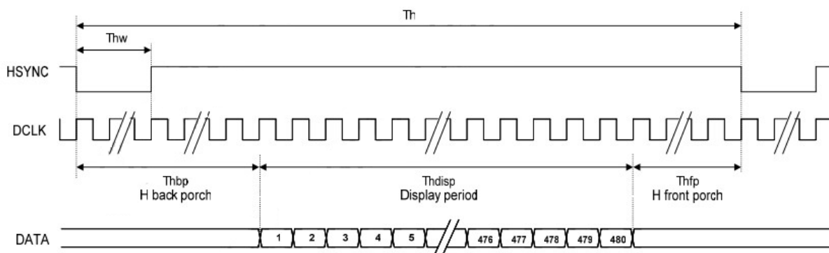
Sync Mode Timing Diagram
