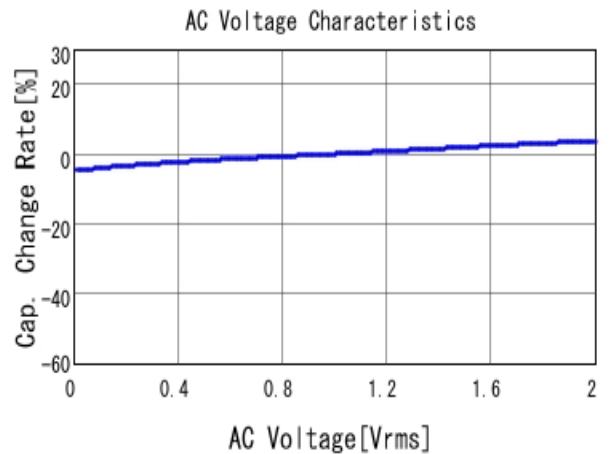
■ GCM219R71E474KA55 C-AC Voltage capchange, DC0V, 25.0d
