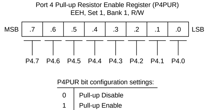
Figure 9-15. Port 4 Pull-up Resistor Enable Register (P4PUR)
