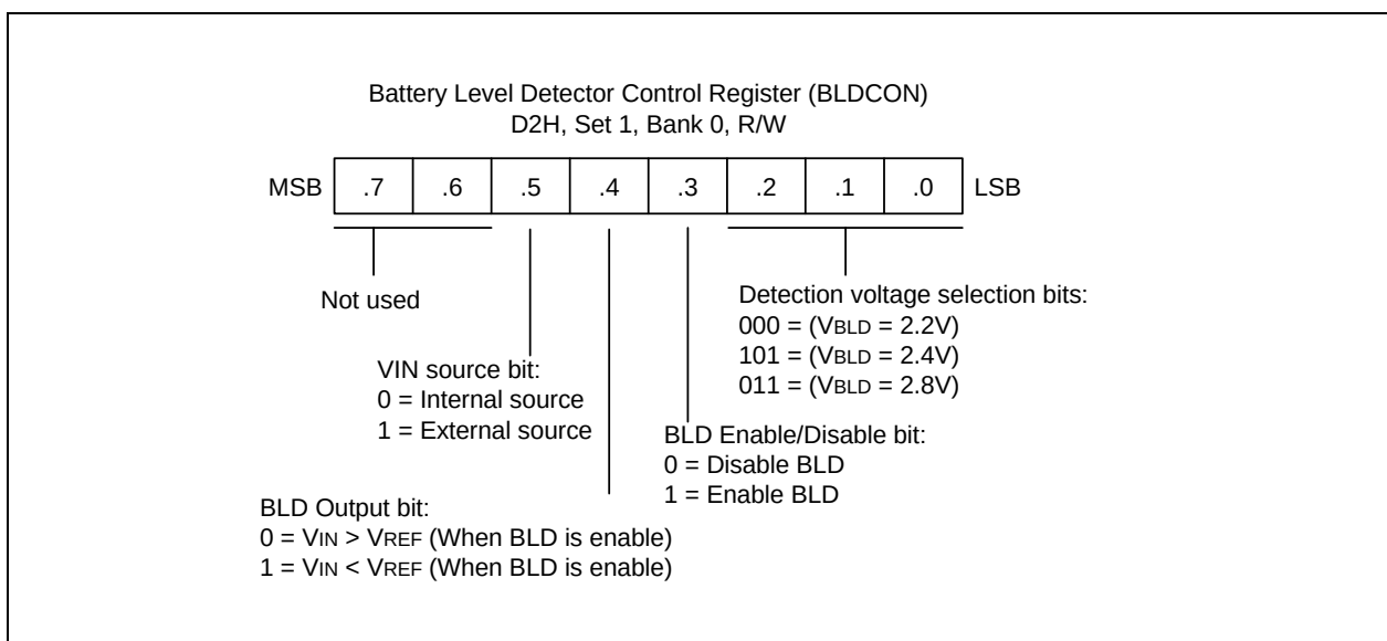
Figure 18-2. Battery Level Detector Control Register (BLDCON)
