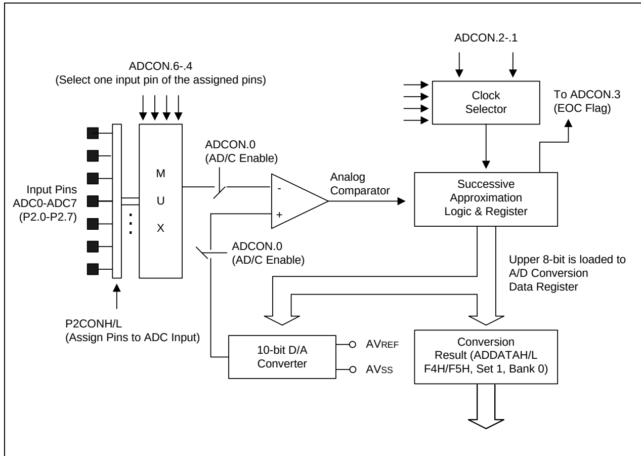
Figure 15-3. A/D Converter Functional Block Diagram
