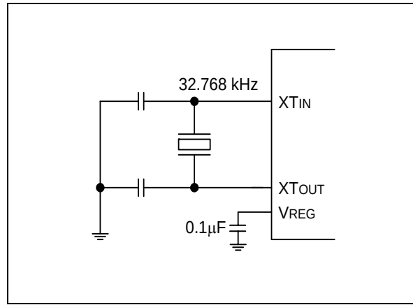
Figure 7-4. Crystal Oscillator (fxt)
