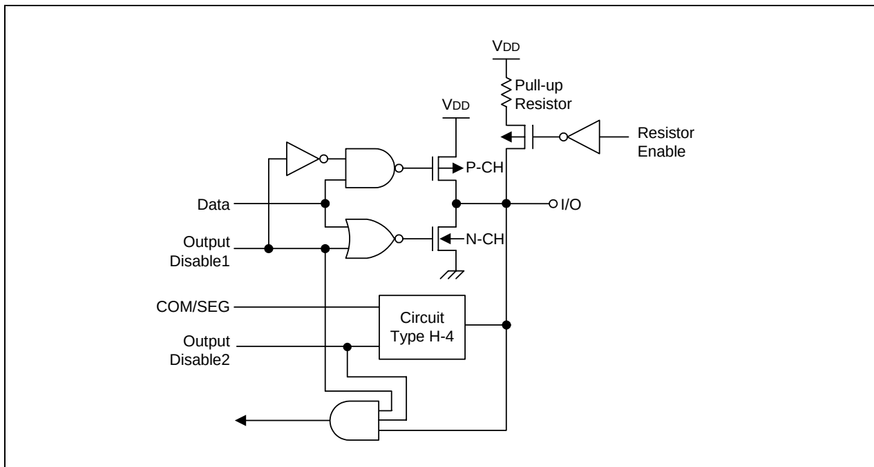
Figure 1-13. Pin Circuit Type H-9 (P3.0-P3.3, P6, P7, P8)
