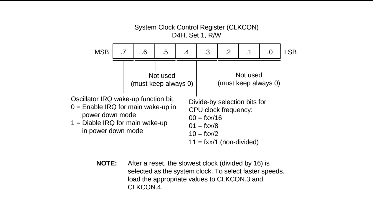
Figure 7-7. System Clock Control Register (CLKCON)
