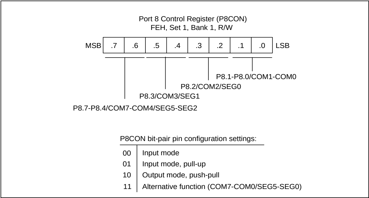
Figure 9-22. Port 8 Control Register (P8CON)
