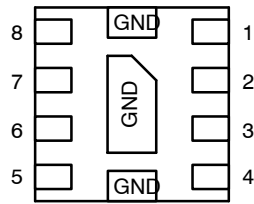
Figure 3. Pin Diagram
