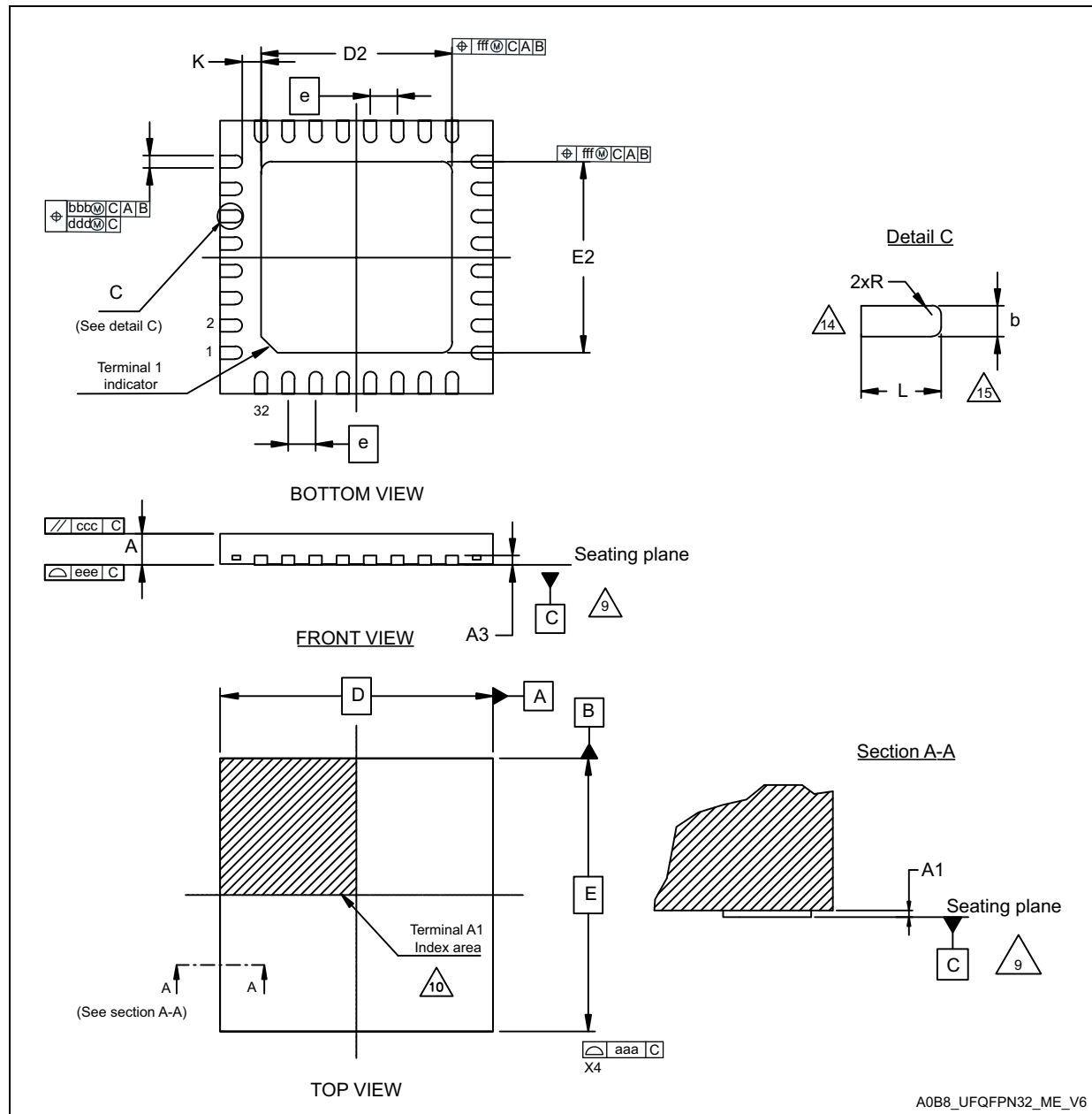
Figure 40. UFQFPN32 - Outline
