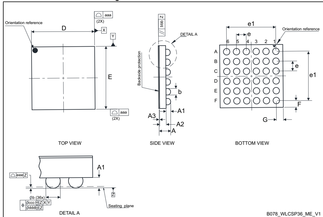
Figure 42. WLCSP36 - Outline
