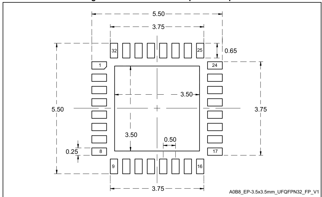
Figure 41. UFQFPN32 - Footprint example
