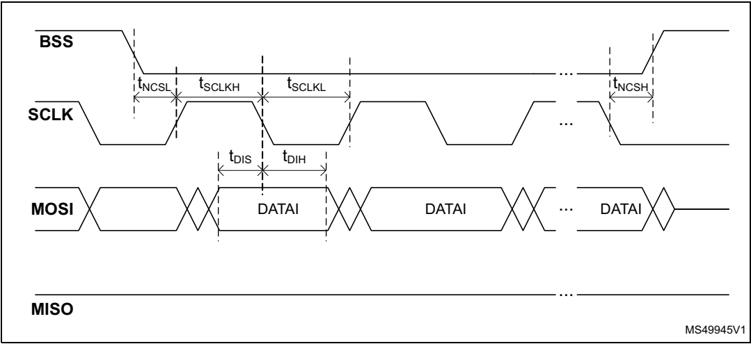
Figure 32. SPI timing diagram - General operation
