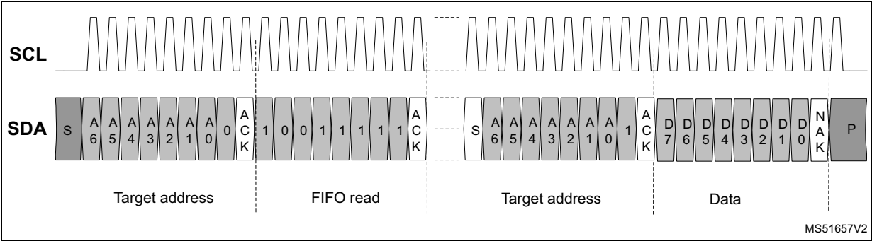
Figure 26. FIFO read
