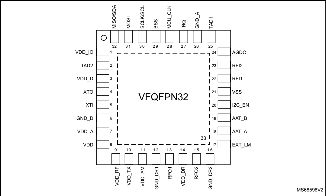
Figure 4. ST25R3916B QFN32 pinout (top view)
