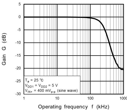
Fig. 12.11 G[\text{dB}] - f
