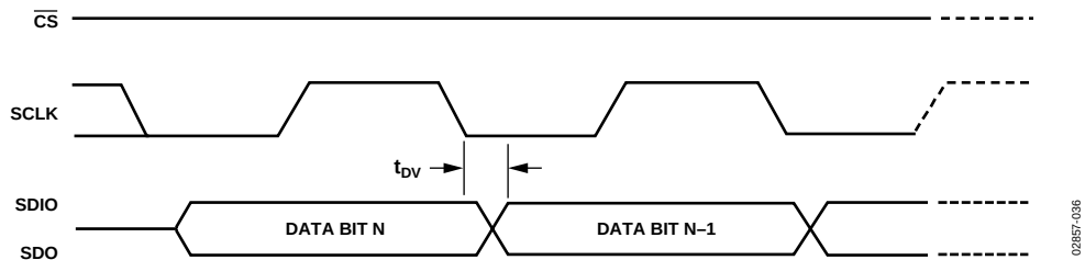
Figure 36. Timing Diagram for Register Read from AD9773
