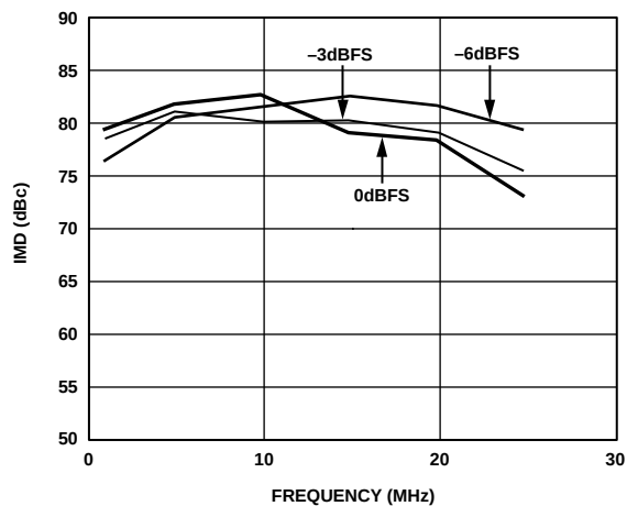
Figure 15. Third-Order IMD Products vs. f_{OUT} @ f_{DATA} = 65 MSPS
