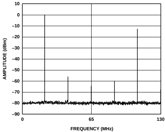
Figure 6. Single-Tone Spectrum @ f_{DATA} = 65\text{ MSPS} with f_{OUT} = f_{DATA}/3
