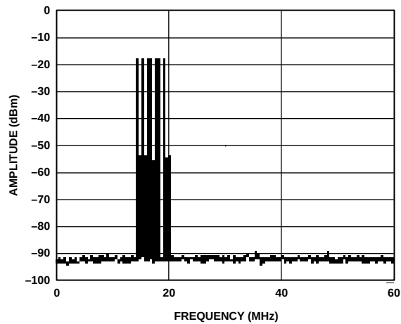
Figure 31. Eight-Tone IMD Performance, f_{DATA} = 160 MSPS, Interpolation = 8 \times
