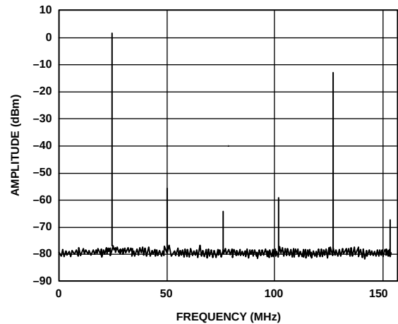
Figure 9. Single-Tone Spectrum @ f_{DATA} = 78\text{ MSPS} with f_{OUT} = f_{DATA}/3
