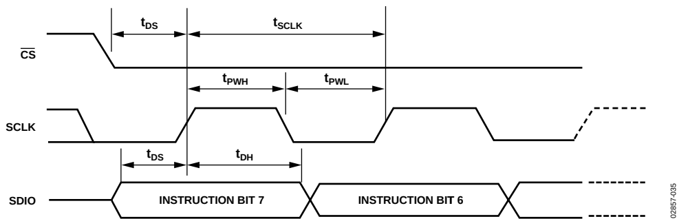
Figure 35. Timing Diagram for Register Write to AD9773
