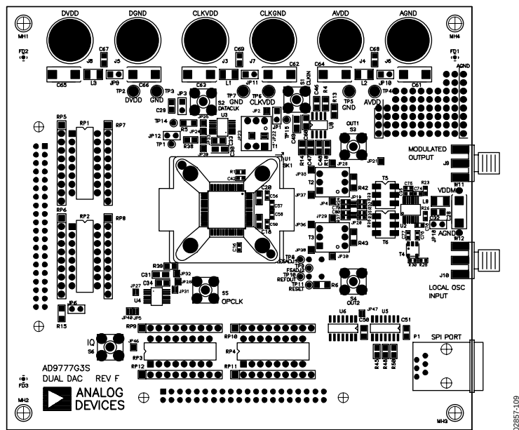
Figure 109. AD9773 Evaluation Board Components, Top Side
