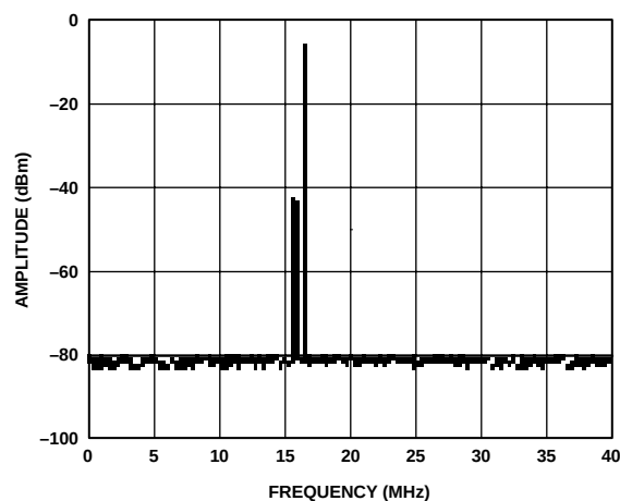
Figure 27. Two-Tone IMD Performance, f_{DATA} = 150 MSPS, Interpolation = 4x
