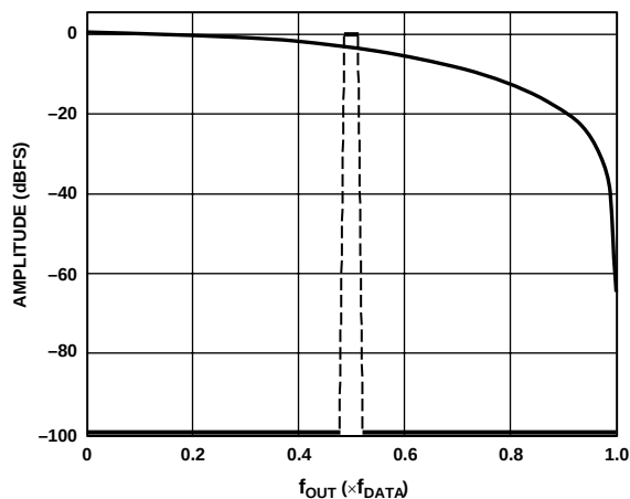
Figure 60. No Interpolation, Modulation = f_{\text{DAC}}/2
