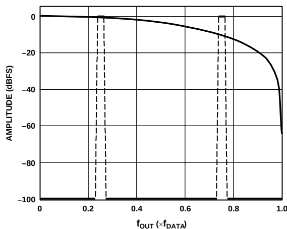
Figure 61. No Interpolation, Modulation = f_{\text{DAC}}/4
