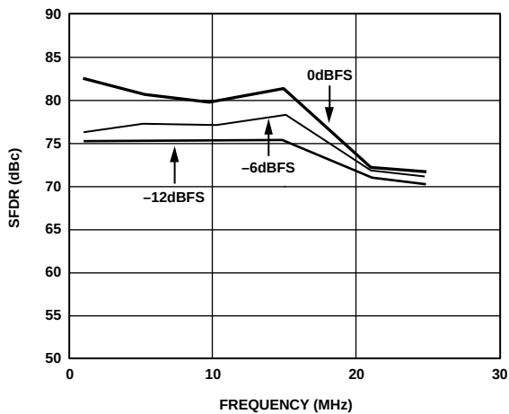
Figure 7. In-Band SFDR vs. f_{OUT} @ f_{DATA} = 65\text{ MSPS}
