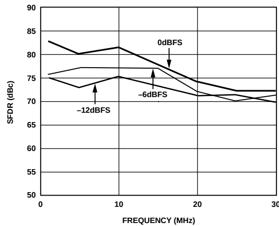
Figure 10. In-Band SFDR vs. f_{OUT} @ f_{DATA} = 78\text{ MSPS}
