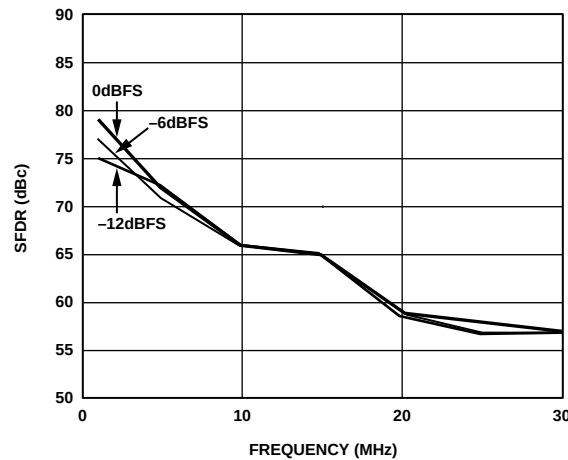
Figure 11. Out-of-Band SFDR vs. f_{OUT} @ f_{DATA} = 78\text{ MSPS}
