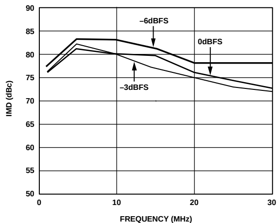
Figure 16. Third-Order IMD Products vs. f_{OUT} @ f_{DATA} = 78 MSPS
