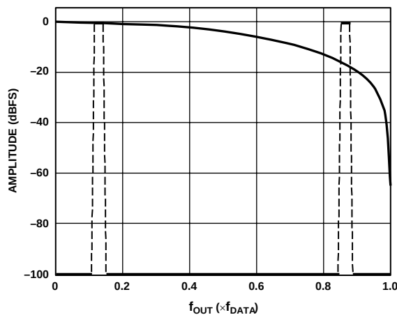
Figure 62. No Interpolation, Modulation = f_{\text{DAC}}/8
