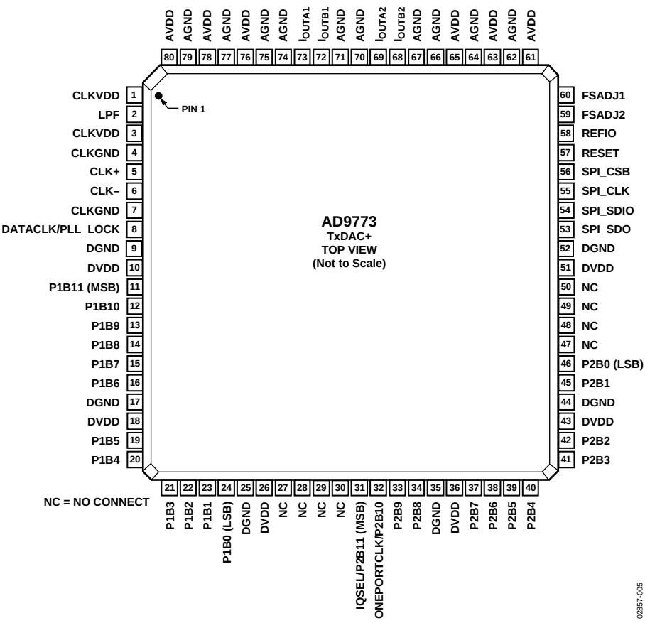
Figure 5. Pin Configuration
