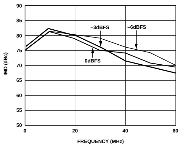
Figure 17. Third-Order IMD Products vs. f_{OUT} @ f_{DATA} = 160 MSPS
