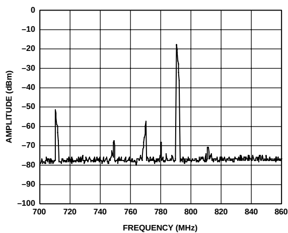
Figure 96. AD9773 Complex Output from Figure 95, Now Quadrature Modulated by AD8345 (LO = 800 MHz)
