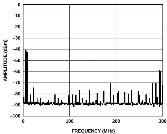
Figure 30. Single-Tone Spurious Performance, f_{OUT} = 10 MHz, f_{DATA} = 50 MSPS, Interpolation = 8 \times
