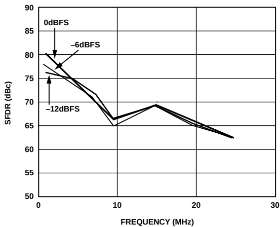
Figure 8. Out-of-Band SFDR vs. f_{OUT} @ f_{DATA} = 65\text{ MSPS}
