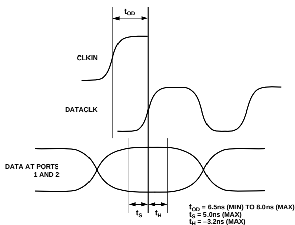
Figure 55. Timing Requirements in Two-Port Input Mode with PLL Disabled
