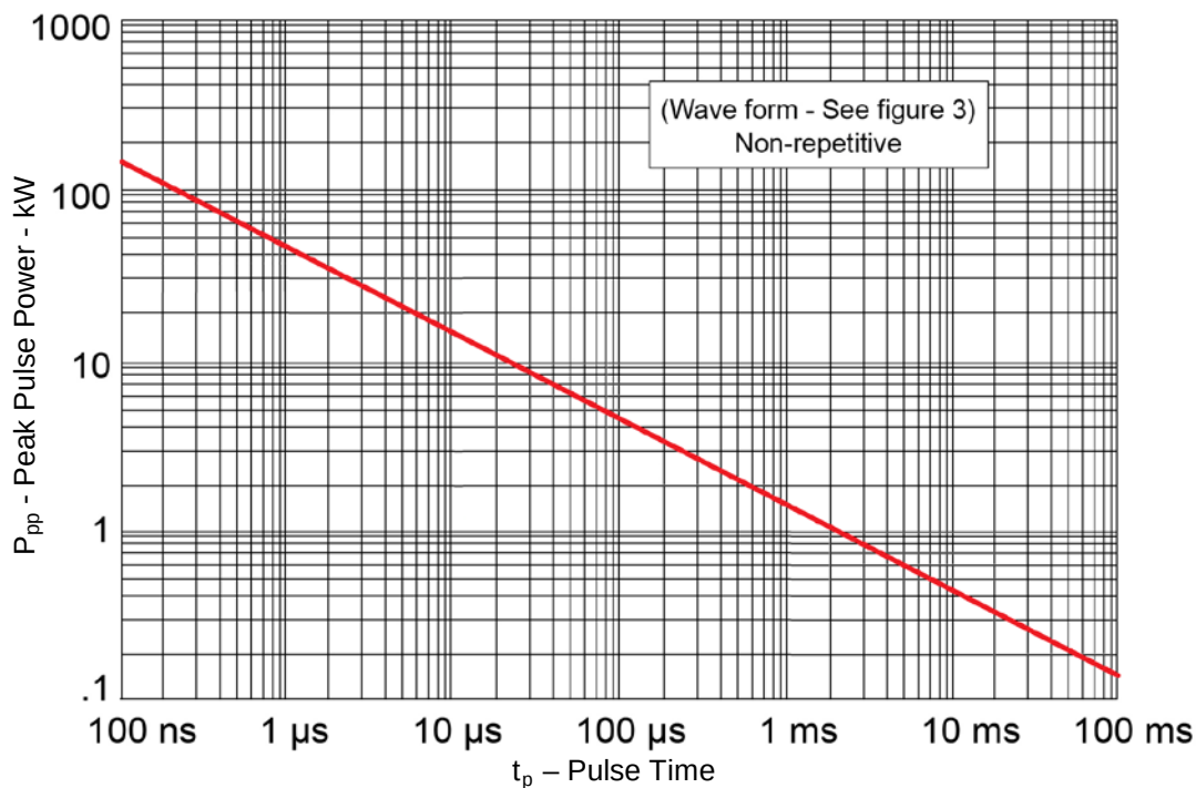
FIGURE 1 Peak Pulse Power vs Pulse Time
