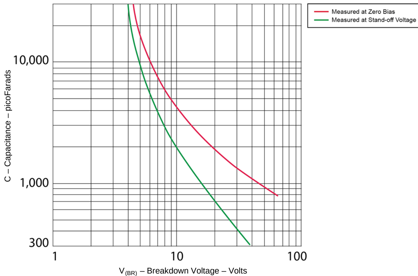
FIGURE 5 Typical Capacitance vs. Breakdown Voltage (Bidirectional Types)
