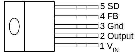
TO220-5L/TO220-5L(R)
