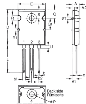
TO-264 (IXTK) Outline
