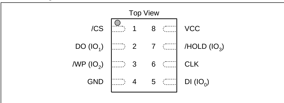
Figure 1a. W25N01GW Pad Assignments, 8-pad WSON 8x6-mm (Package Code ZE)
