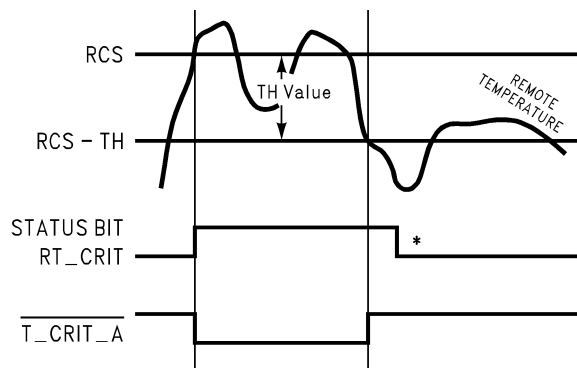
Figure 8. T_CRIT_A Temperature Response Diagram
