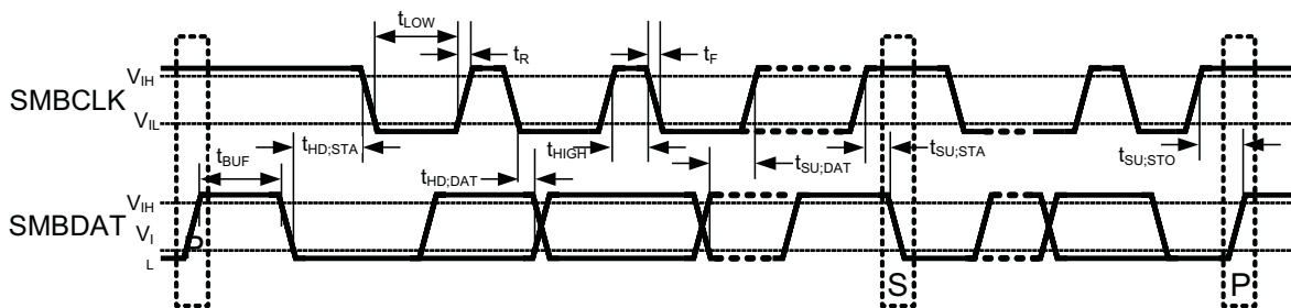
Figure 2. SMBus Communication
