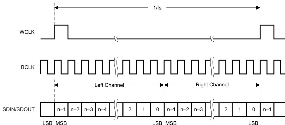
Figure 21. DSP Serial Bus Mode Operation
