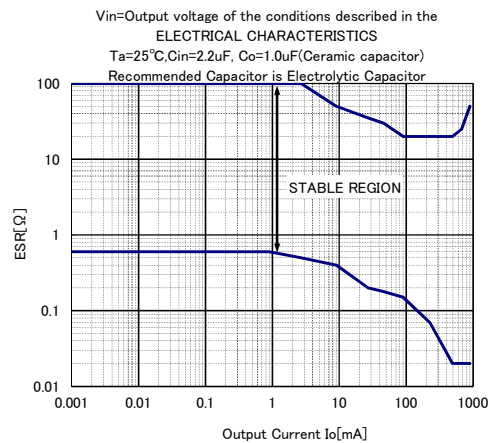
NJM7900 Equivalent Series Resister Vs. Output Current
