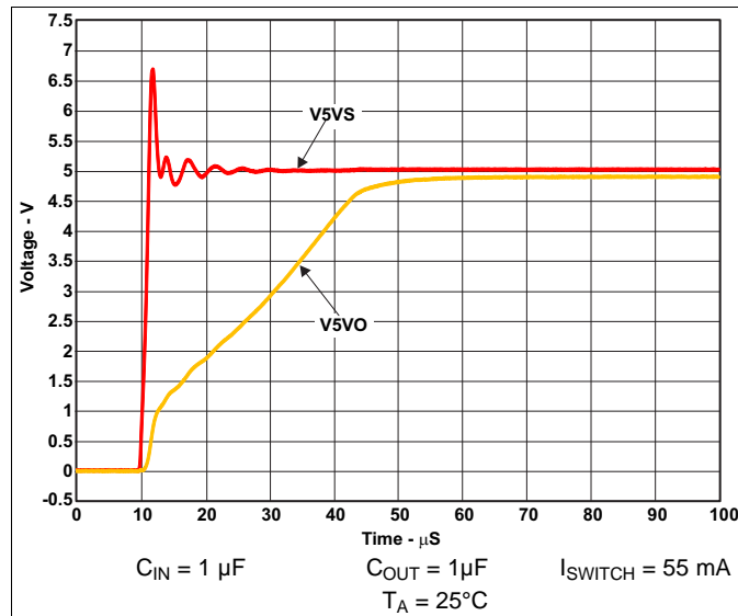
Figure 7. Load Switch Start-Up Transient Waveform
