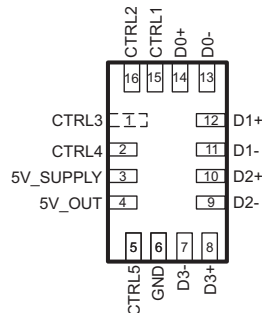
RSV Package 16-Pin UQFN Top View
