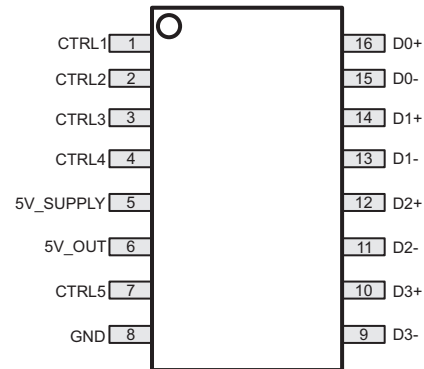
PW Package 16-Pin TSSOP Top View
