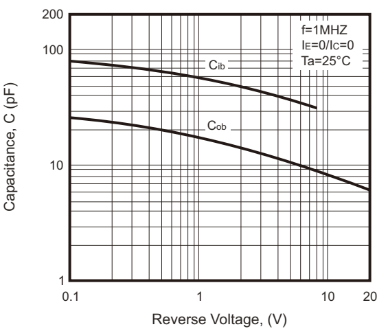
Fig.6 - C_{ob}/C_{ib} - V_{CB}/V_{EB}
