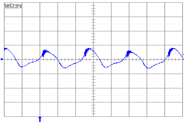
Figure 10. Output voltage ripple (20 mV/div.) at full rated load current into a resistive load with C_o = 10 \mu F tantalum + 1 \mu F ceramic and V_{in} = 48 V. Time scale: 1 \mu s/div.
