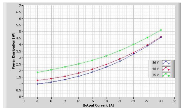
Figure 3. Power dissipation vs. load current and input voltage for SQE48T30010 converter mounted horizontally. Convection cooled with T_a = 25^\circ\text{C} .
