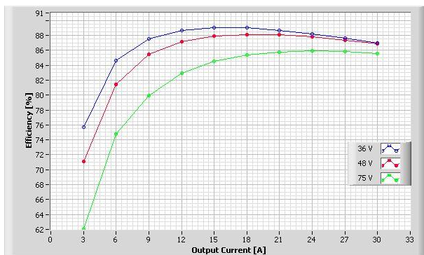
Figure 2. Efficiency vs. load current and input voltage for SQE48T30010 converter mounted horizontally. Convection cooled with T_a = 25^\circ\text{C} .
