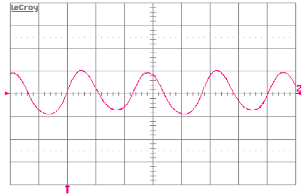
Figure 13. Input reflected ripple-current, i_c (100 mA/div.), measured at input terminals at full rated load current and V_{in} = 48\ \text{V} . Refer to Fig. 12 for test setup. Time scale: 1\ \mu\text{s}/\text{div} .
