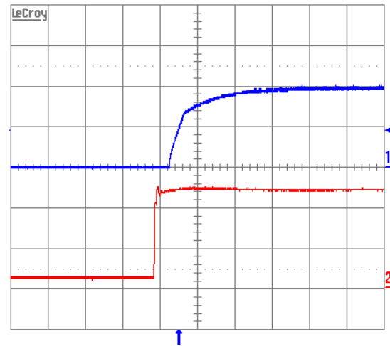
Figure 5. V_{in} versus output voltage for SQE48T30010 converter mounted horizontally. V_{in}=48\text{Vdc} , I_{out}=30\text{Amps} , C_{out}=10,000\mu\text{F} and turned on using V_{cc} . Convection cooled with T_a=25^\circ\text{C} . Top trace: Output voltage (0.5 V/div.). Bottom trace: V_{CC} (20 V/div.). Time scale: 2 ms/div. Convection cooled with T_a=25^\circ\text{C} .
