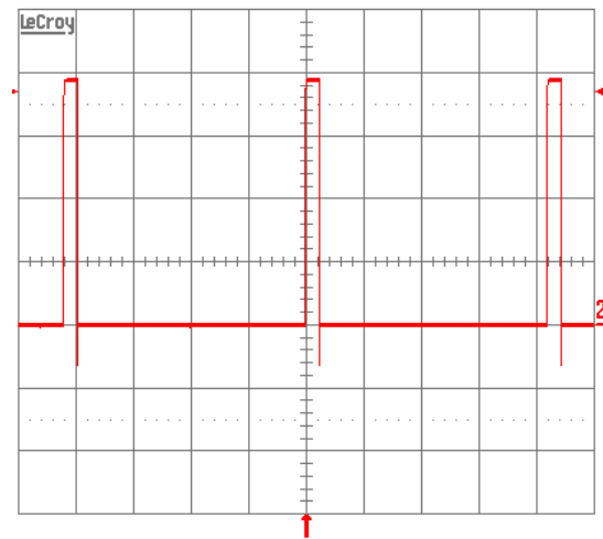
Figure 15. Load current (top trace, 10 A/div., 50 ms/div.) into a 10\ \text{m}\Omega short circuit during restart, at V_{in} = 48\ \text{V} .
