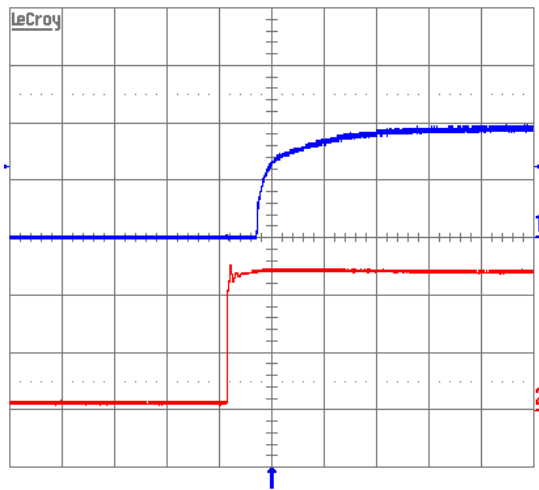
Figure 4. V_{in} versus output voltage for SQE48T30010 converter mounted horizontally. V_{in}=48\text{Vdc} , I_{out}=30\text{Amps} and turned on using V_{cc} . Top trace: Output voltage (0.5 V/div.). Bottom trace: V_{CC} (20 V/div.). Time scale: 2 ms/div. Convection cooled with T_a=25^\circ\text{C} .
