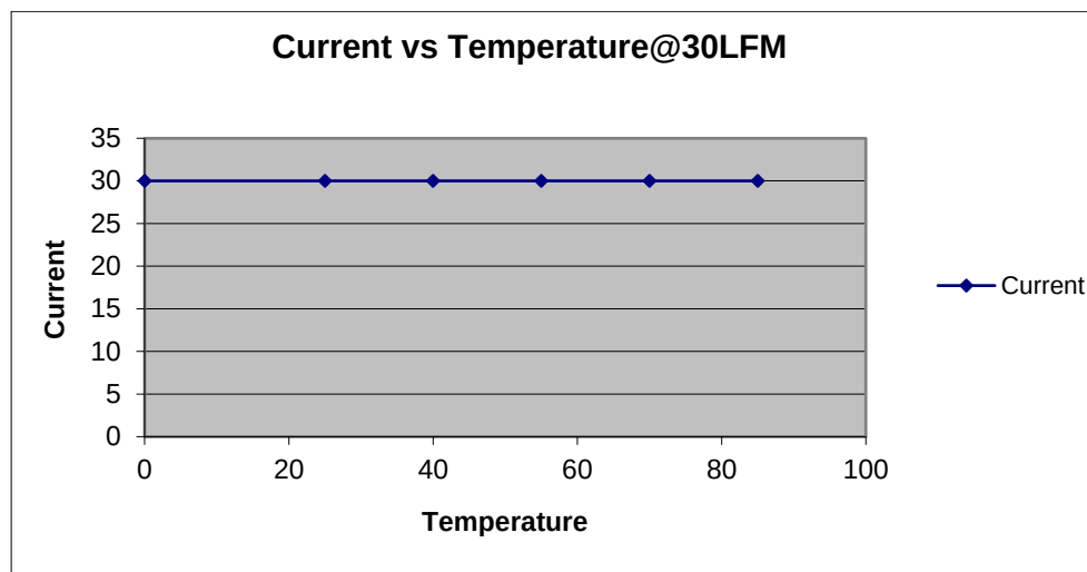
Figure 1. Available load current vs. ambient air temperature for an SQE48T30010 converter mounted vertically with air flowing from pin 3 to pin 1, MOSFET temperature \leq 125^\circ\text{C} , V_{in} = 48\text{ V} .
