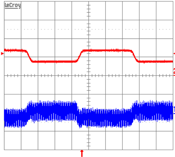
Figure 8. Output voltage response to load current step-change (7.5A – 15A – 7.5A) at V_{in} = 48 V. Top trace: load current (5 A/div.) Bottom trace: output voltage (50 mV/div.). Current slew rate: 0.1 A/ \mu s. C_o = 1 \mu F ceramic. Time scale: 0.1 ms/div.
