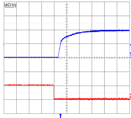
Figure 7. Turn-on transient at full rated load current (resistive) plus 10,000 \mu\text{F} at V_{in} = 48\text{V} , 30 Amps and turned on using ON/OFF pin. Top trace, I_{out} =Output voltage (0.5 V/div.). Bottom trace: ON/OFF signal (5 V/div.). Time scale: 2 ms/div.
