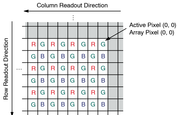
Figure 6. RGB Pixel Color Pattern Detail (Top Right Corner) – AR0141CS
