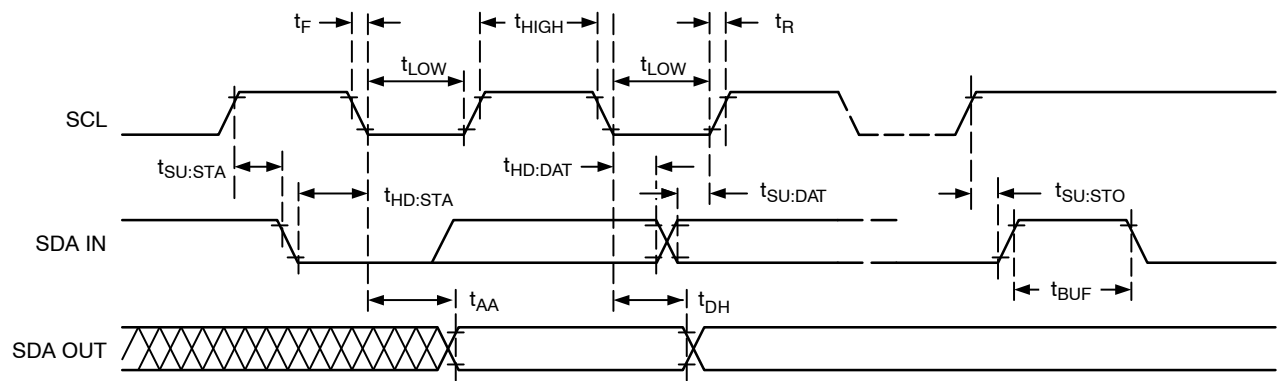
Figure 8. Bus Timing
