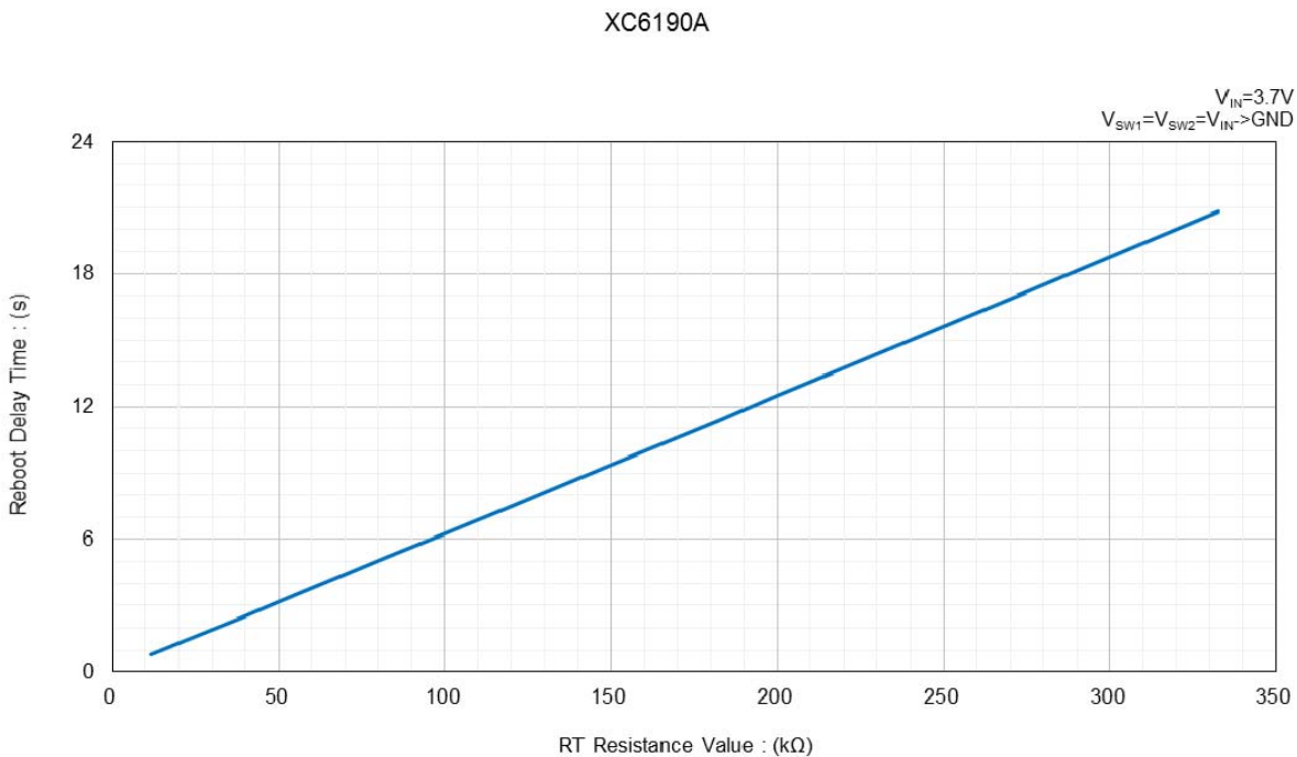
(13) Reboot Delay Time vs. RT Resistance Value
