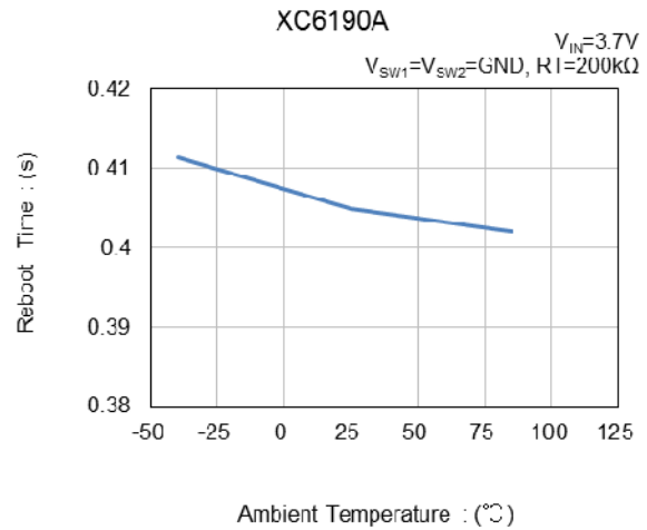
(12) Reboot Time vs. Ambient Temperature
