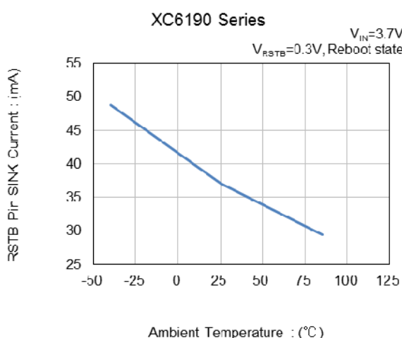
(10) RSTB pin SINK Current vs. Ambient Temperature
