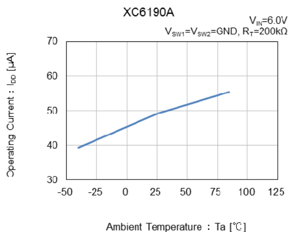
(4) Operating Current vs. Ambient Temperature
