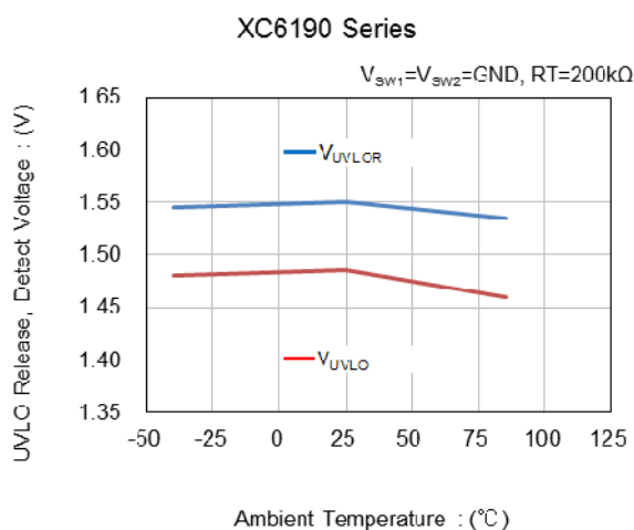
(5) UVLO Release, Detect Voltage vs. Ambient Temperature
