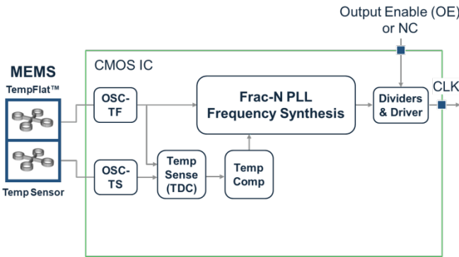
Figure 35. Block Diagram – TCXO
