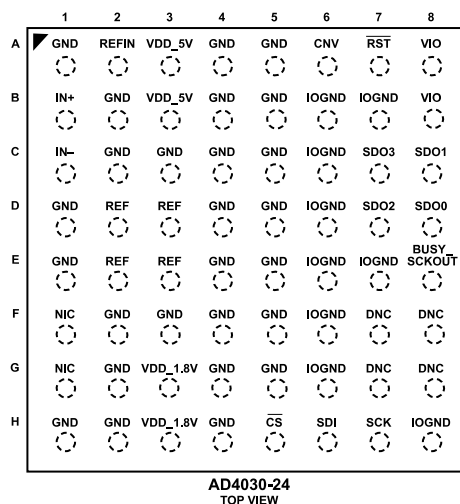
Figure 11. Pin Configuration
