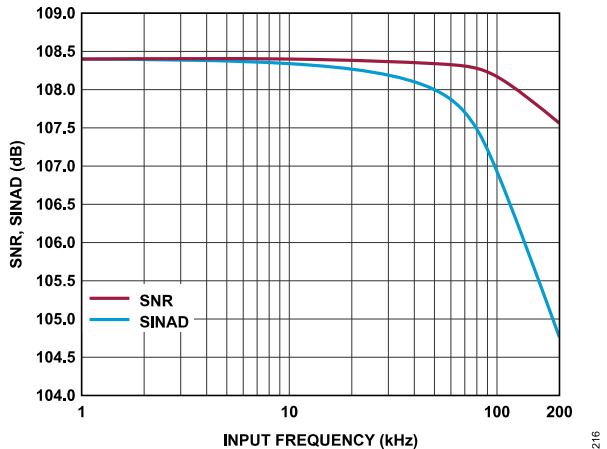
Figure 16. SNR, SINAD vs. Input Frequency
