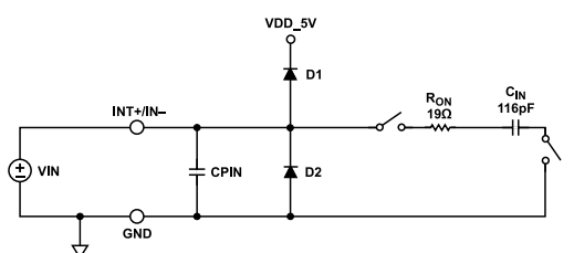
Figure 38. Equivalent Circuit for the AD4030-24 Differential Analog Input
