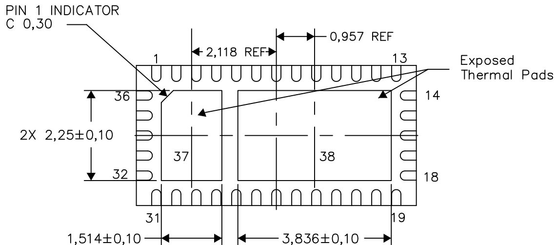
Bottom View
