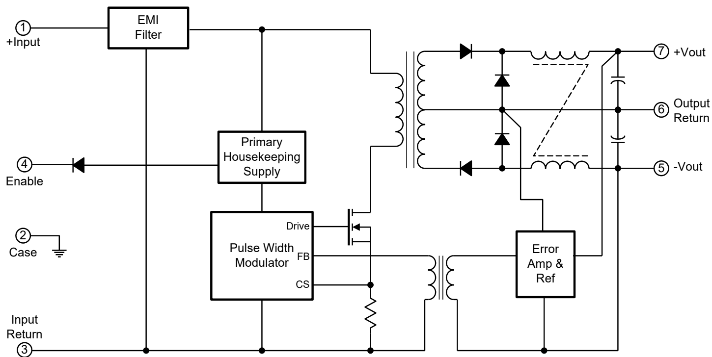
Figure 2. Block Diagram - Dual Output
